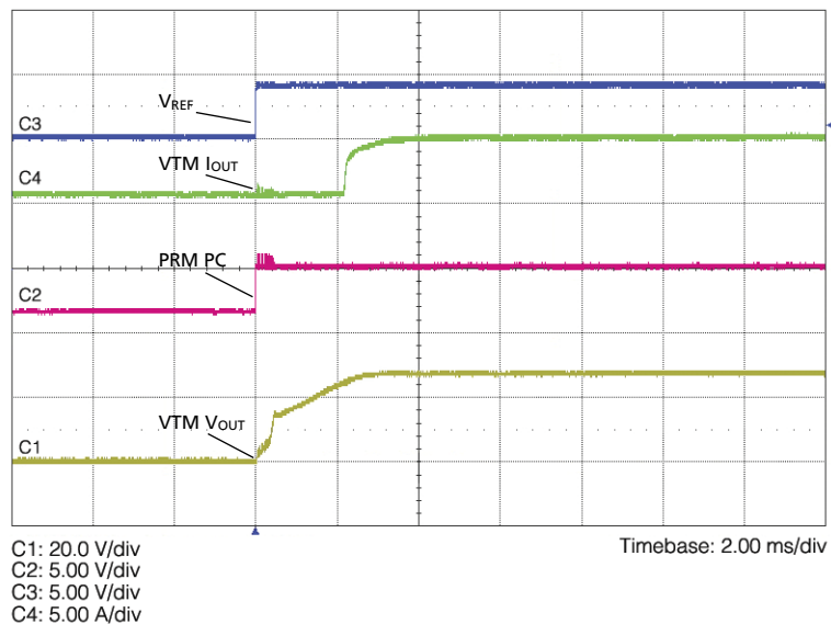
Figure 16 Electronic Load Constant Resistance PRM – VTM Start Up Waveform
