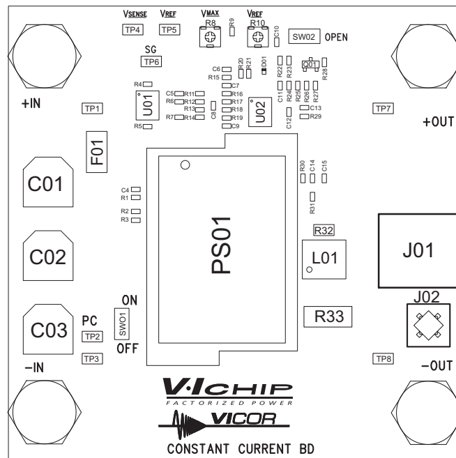
Figure 3 CC Demonstration Board Layout
