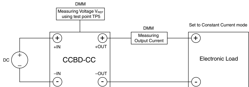
Figure 9 CC Electronic / Resistive Load
