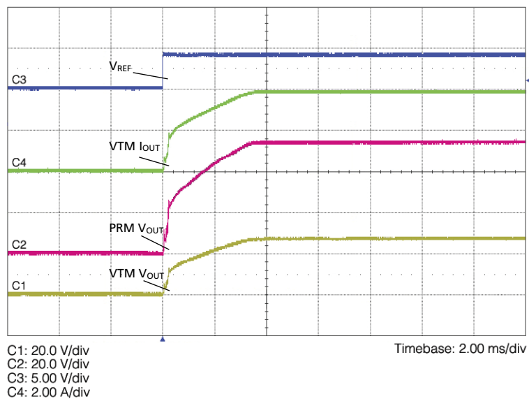
Figure 17 Resistive Load PRM – VTM Start Up Waveform
