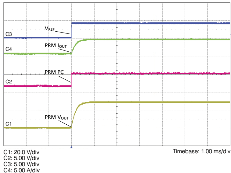
Figure 13 Resistive Load PRM Start Up Waveform
