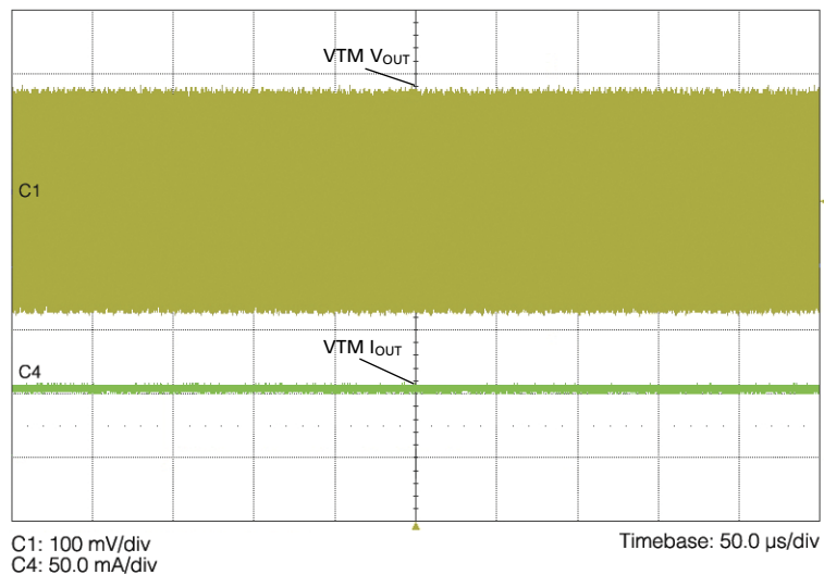
Figure 19 Resistive Load PRM – VTM V_{OUT} & I_{OUT} Ripple
