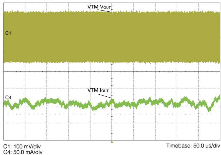
Figure 18 Electronic Load CV PRM – VTM V_{OUT} & I_{OUT} Ripple
