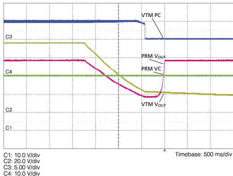
Figure 7 PRM & VTM Under-voltage Abnormal Behavior
