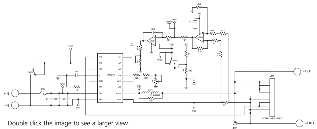
Figure 1 CC Demonstration Board Schematic
