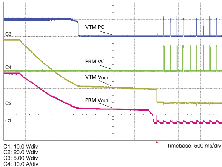
Figure 6 PRM & VTM Under-voltage Behavior
