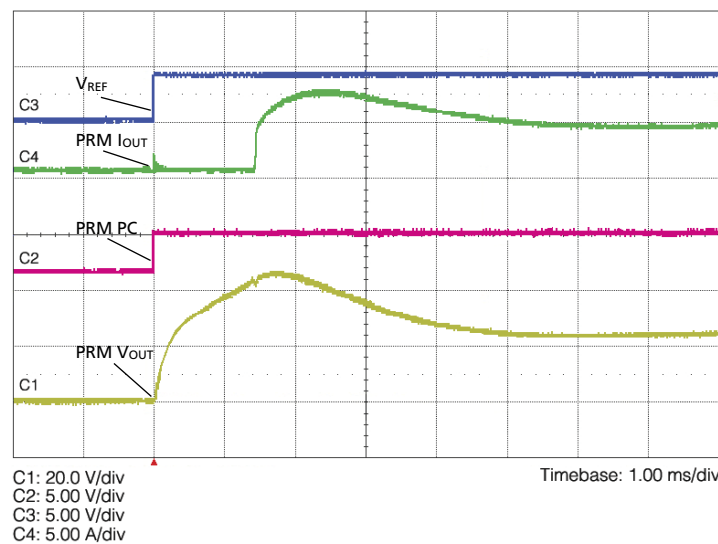
Figure 11 Electronic Load Constant Resistance PRM Start Up Waveform
