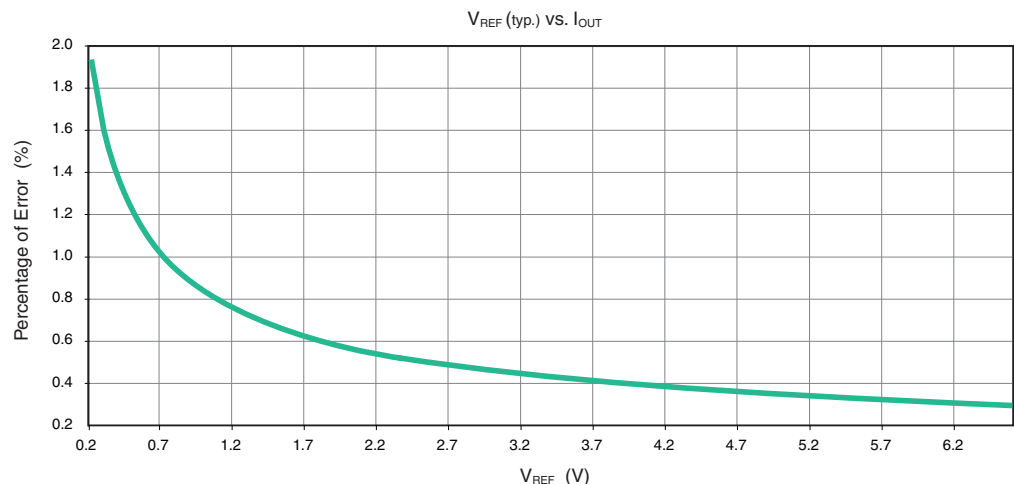
Figure 10 V_{REF} VS. I_{OUT} PRM Error Margin
