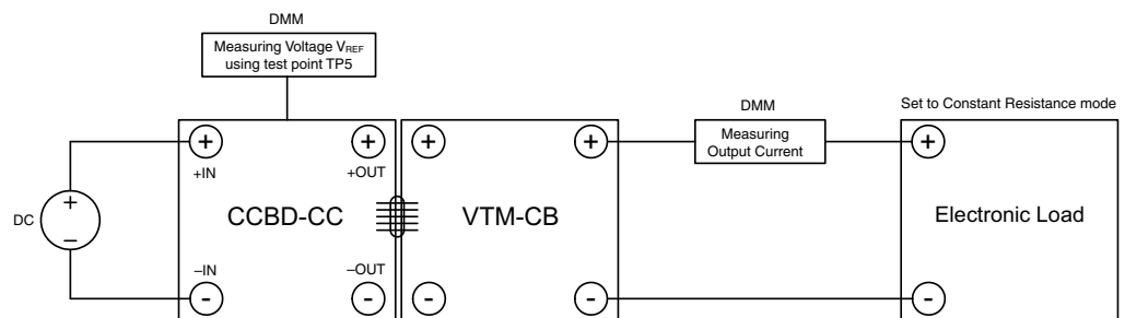
Figure 14 CC & VTM Electronic / Resistive Load
