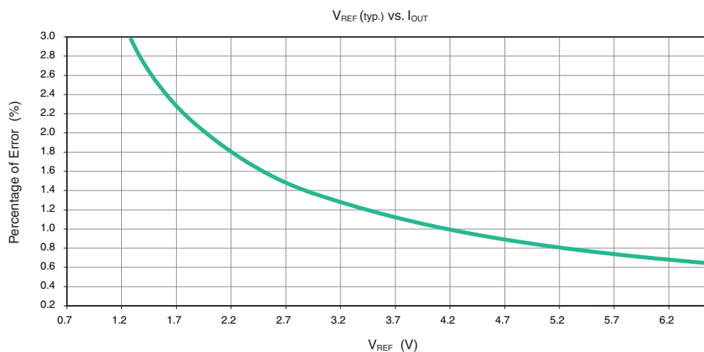
Figure 15 V_{REF} vs. I_{OUT} PRM – VTM Error Margin
