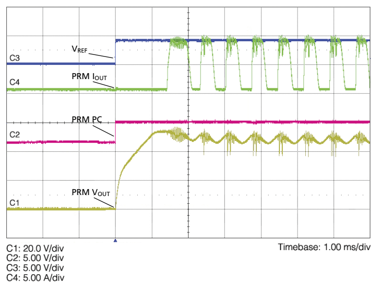
Figure 12 Electronic Load Constant Voltage PRM Start Up Waveform
