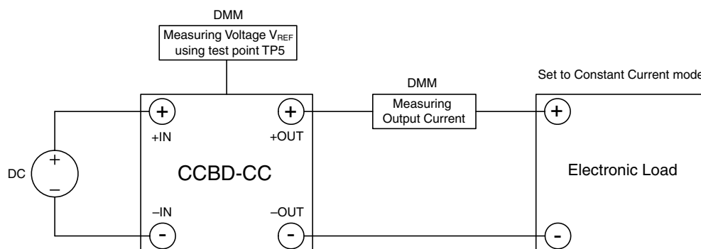
Figure 8 CC No Load Functional Verification
