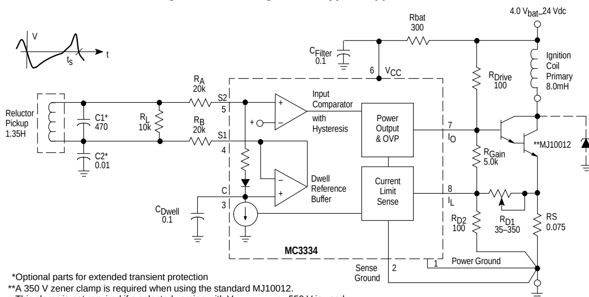
Figure 1. Block Diagram and Typical Application
