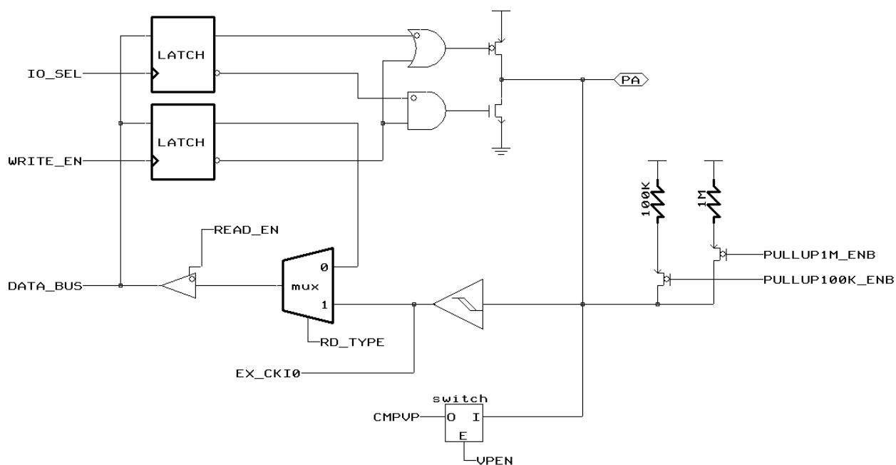
Figure 6 Block Diagram of PA4
