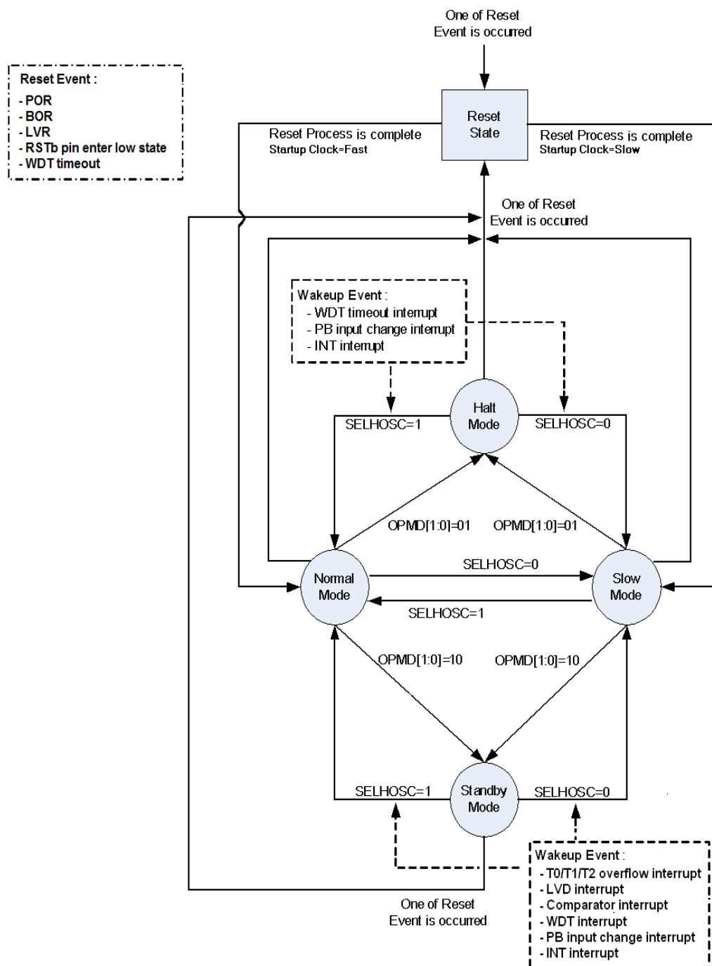
Figure 31 Four Operating Modes
