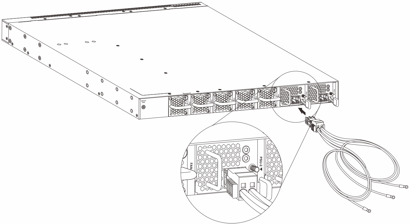
Figure 3-12 Connecting a DC Battery to the DC Power Supply Module
