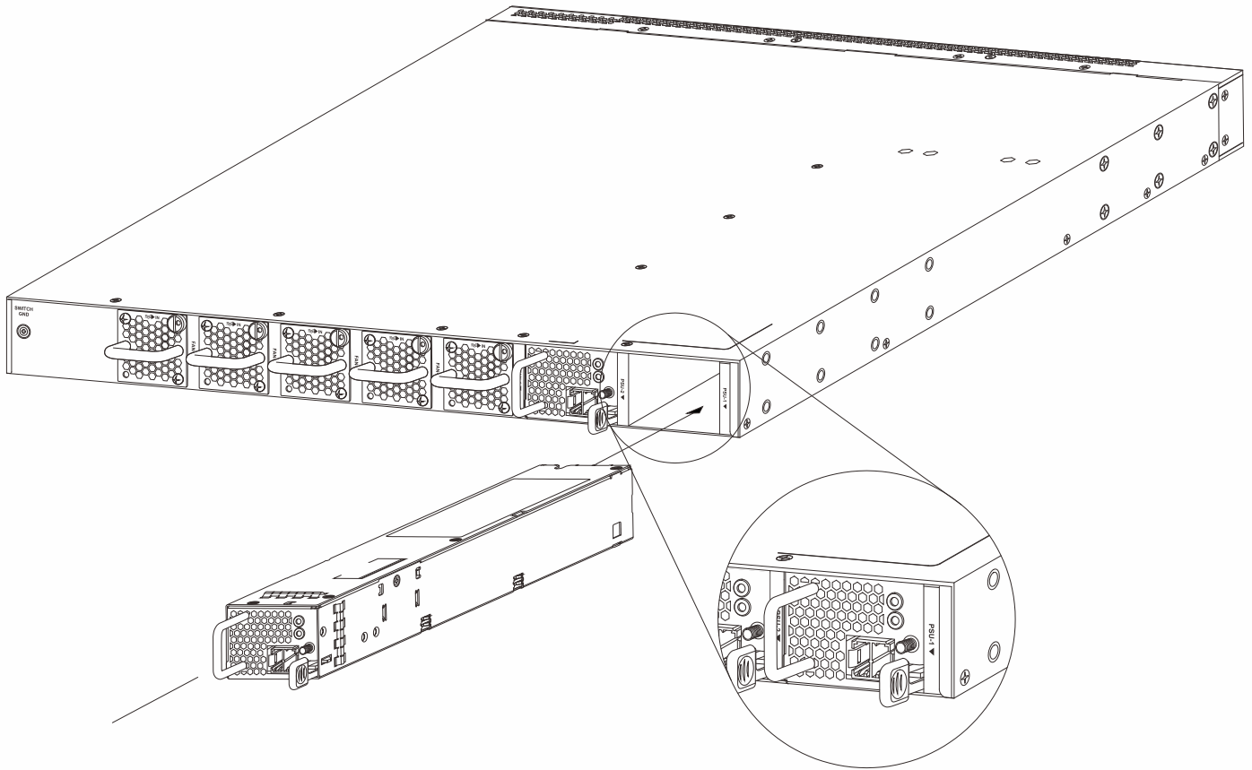
Figure 3-10 Installing a DC PSU Module
