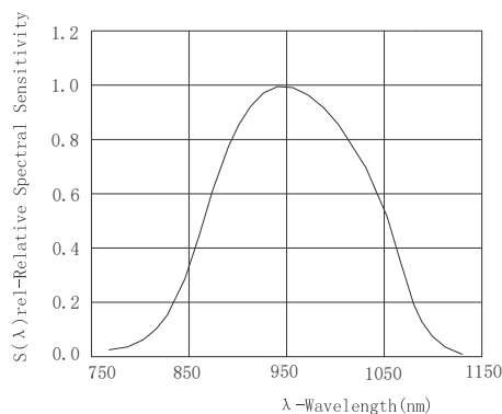
d) Relative Spectral Sensitivity vs. Wavelength
