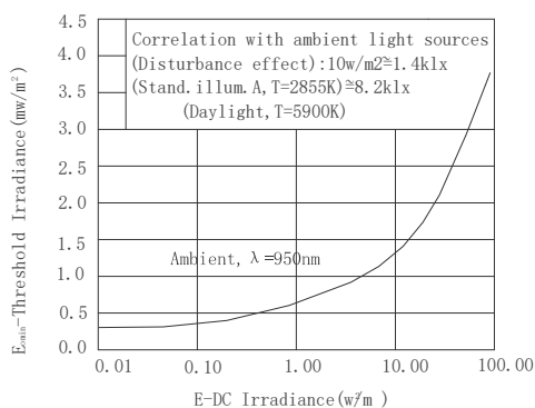
c) Sensitivity in Bright Ambient
