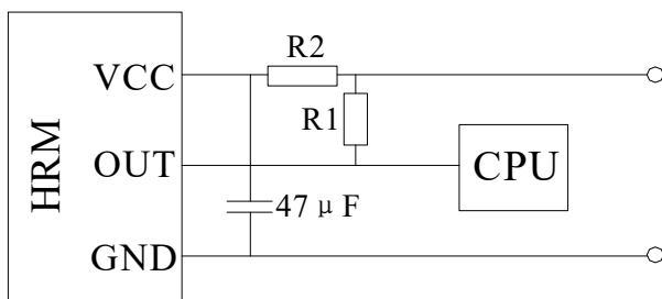
图 12 推荐电路 Figure 12 Recommended Circuit
