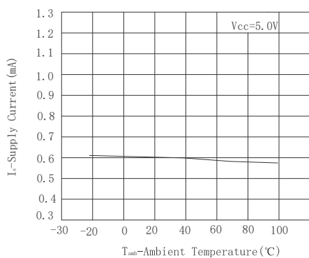
e) Supply Current vs. Ambient Temperature
