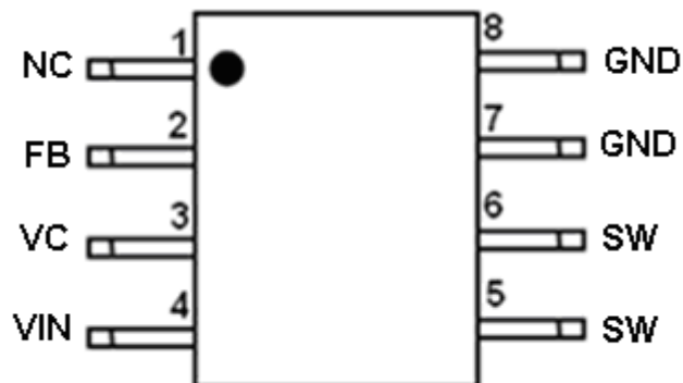
Figure2. Pin Configuration of XL7007 (Top View)
