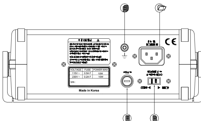
FIG 2-1. REAR PANEL(8102,8103)
