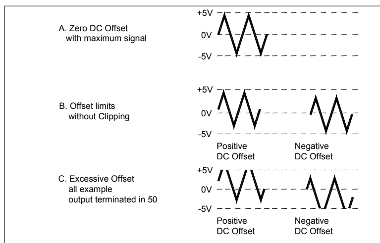
FIG 4. USE OF DC OFFSET CONTROL
