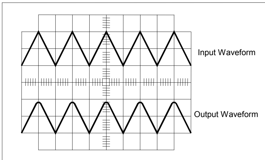
FIG 6. Amplifier overload characteristics
