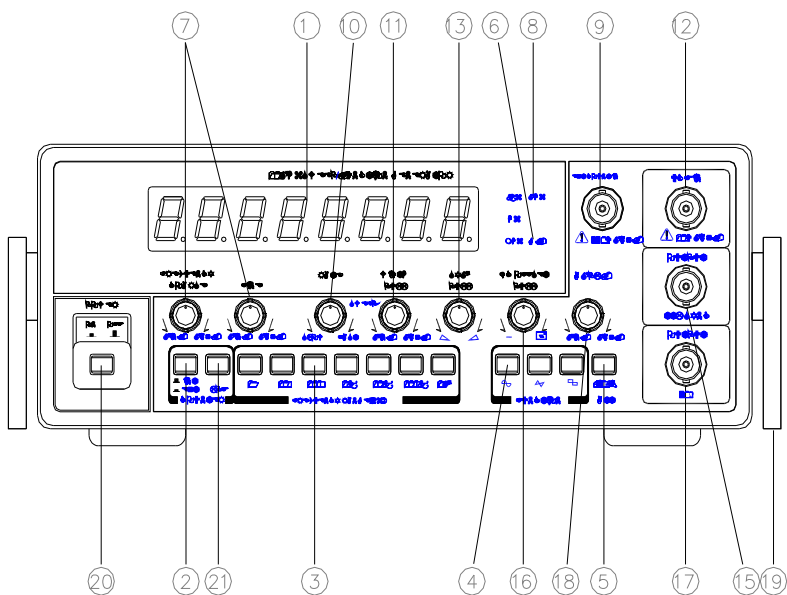
FIG 1-2. FRONT PANEL OPERATOR'S CONTROLS(8105,8110)
