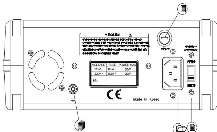
FIG 2-2. REAR PANEL(8105,8110)
