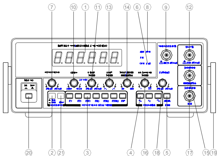
FIG 1-1. FRONT PANEL OPERATOR'S CONTROLS(8102,8103)
