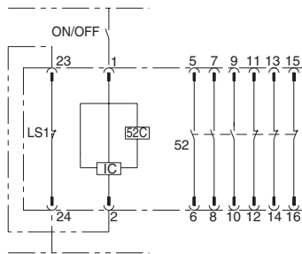
Wiring diagram for external relay circuit (Example)
