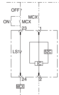
Wiring diagram for external relay circuit (Example)
