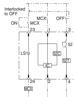
Wiring diagram for external relay circuit (Example)
