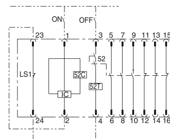
Wiring diagram for external relay circuit (Example)
