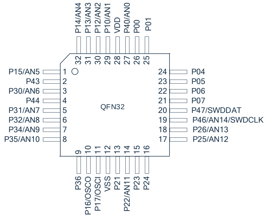
CMS32F030K6T6
