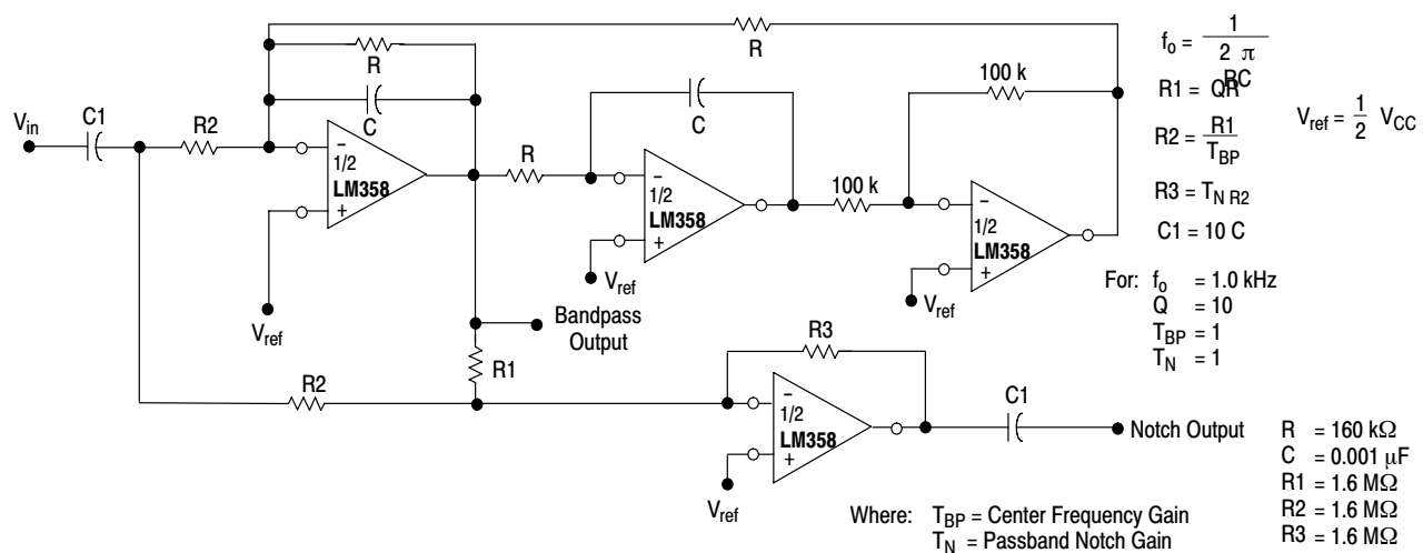
Figure 14. Bi-Quad Filter
