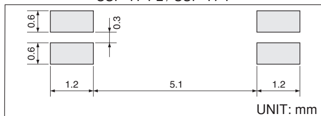
SSP-T7-FL / SSP-T7-F
