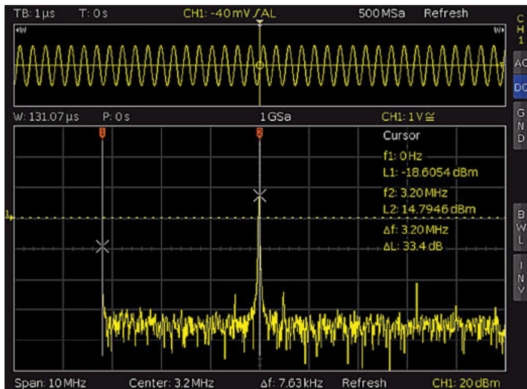
Figure 6-12: FFT
