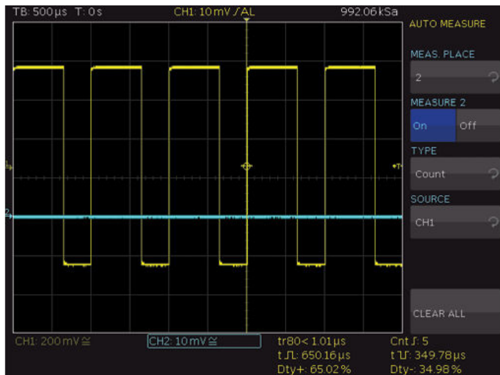
Figure 7-2: Auto measurement settings and results
