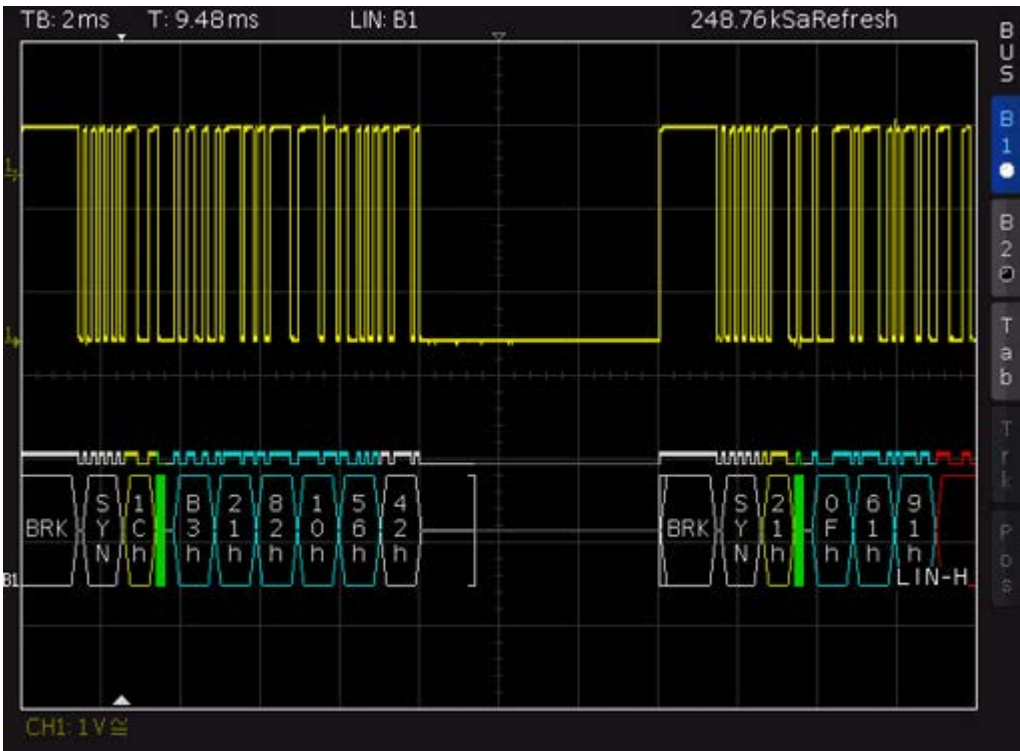
Figure 11-21: LIN bus
