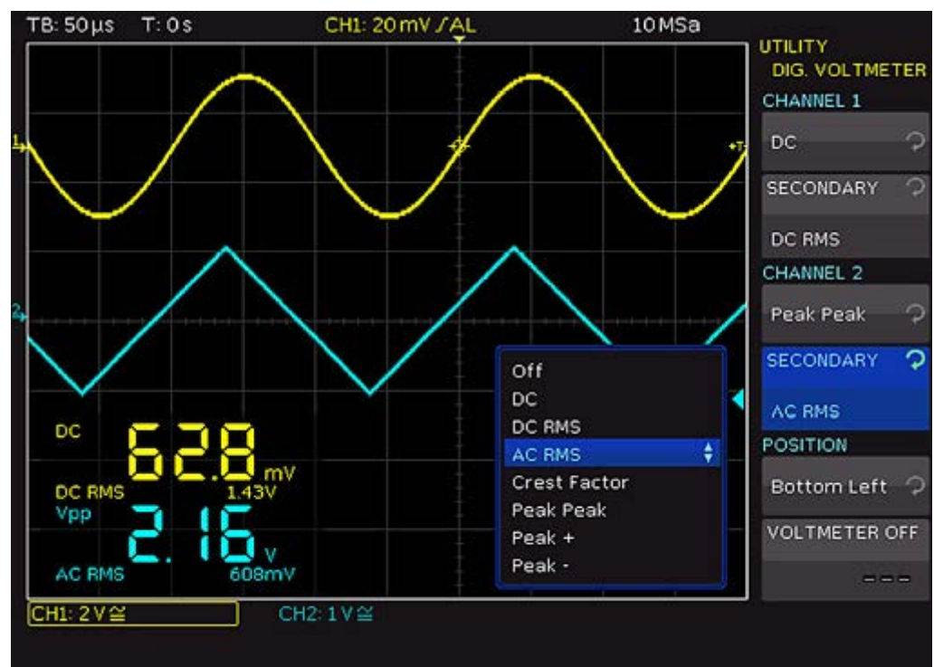
Figure 6-17: Digital Voltmeter
