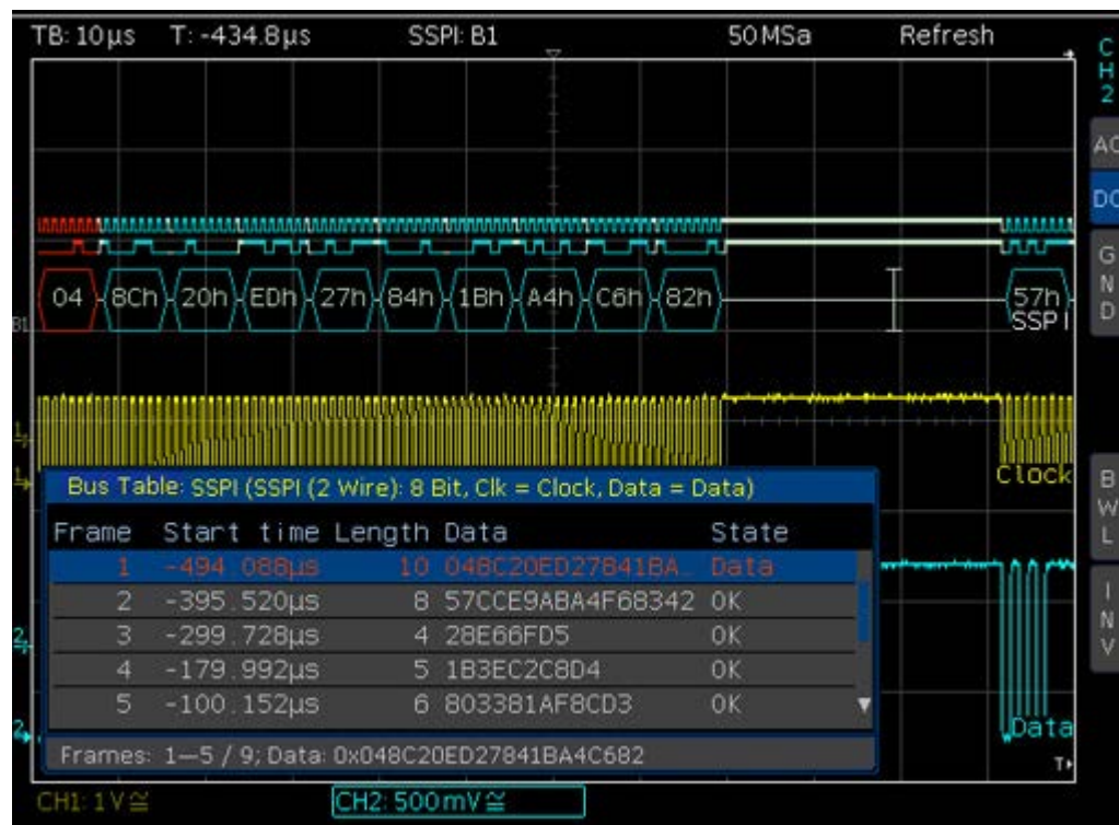
Figure 11-9: Example of an SSPI bus table
