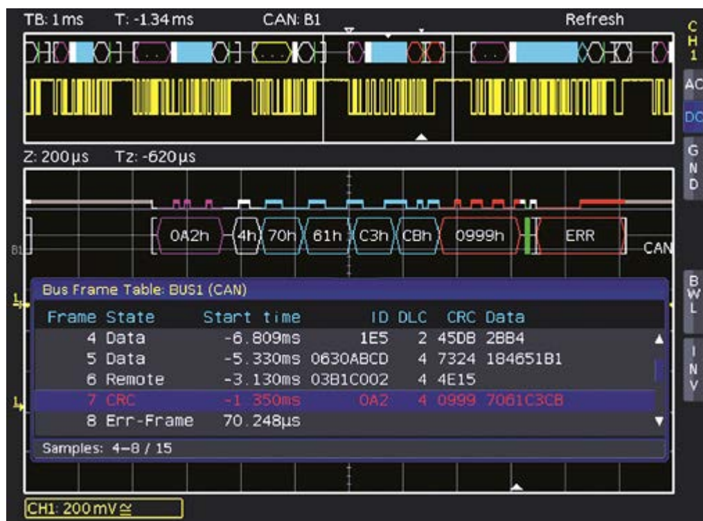
Figure 11-17: Example of a CAN bus table
