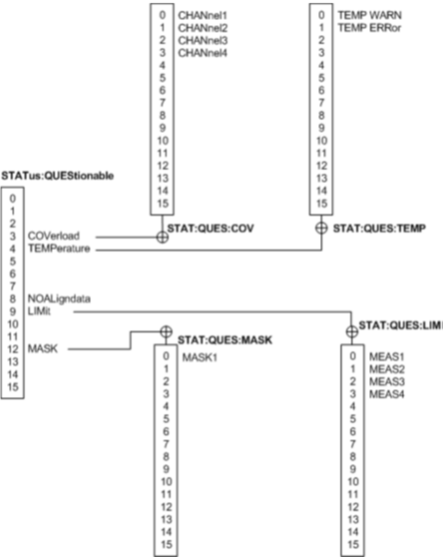
Figure 13-1: Structure of the STATUS:QUESTIONable register
