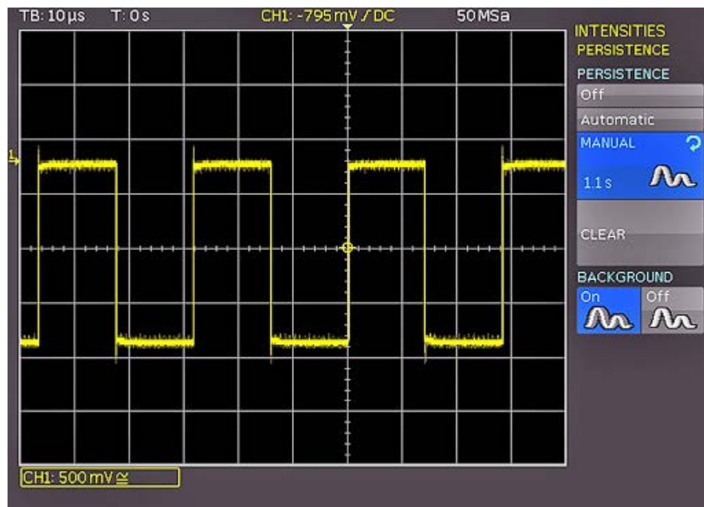
Figure 3-3: Persistence function
