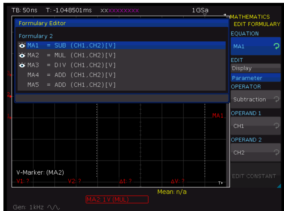
Figure 6-8: Equation parameters (edit equation)
