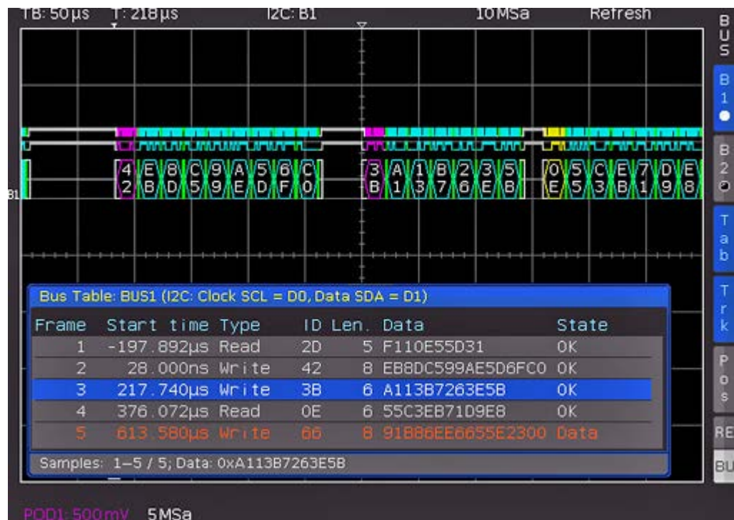
Figure 11-2: Example of I2C BUS with bus table
