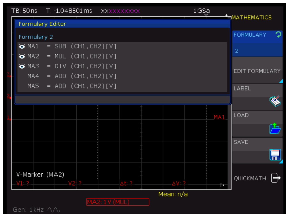
Figure 6-6: Mathematics menu
