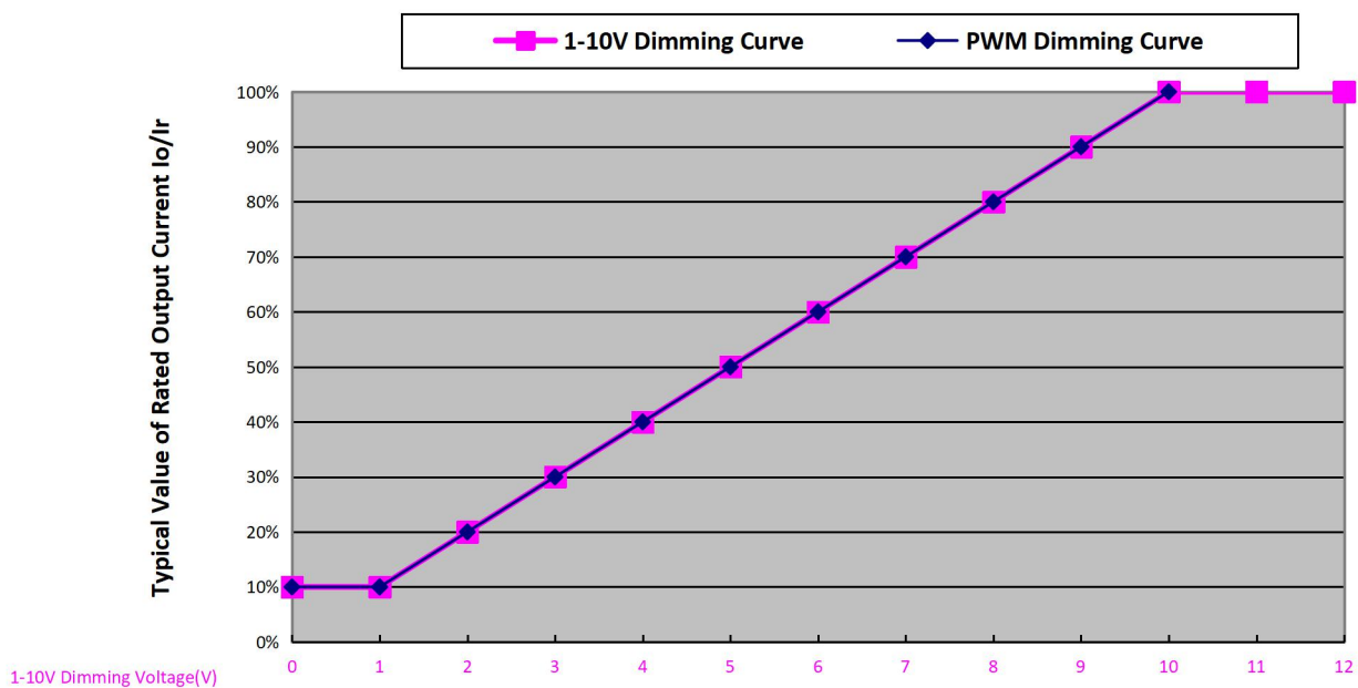
1-10V/PWM Dimming Curve
