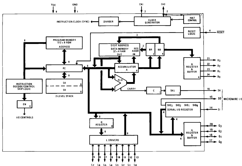
FIGURE 1. COP410C
