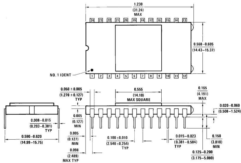
Hermetic Dual-in-Line Package (D) Order Number COP310C-XXX/D, COP411C-XXX/D NS Package Number D24C
