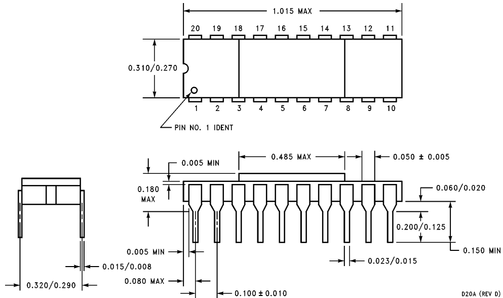
Hermetic Dual-in-Line Package (D) Order Number COP311C-XXX/D, COP411C-XXX/D NS Package Number D20A
