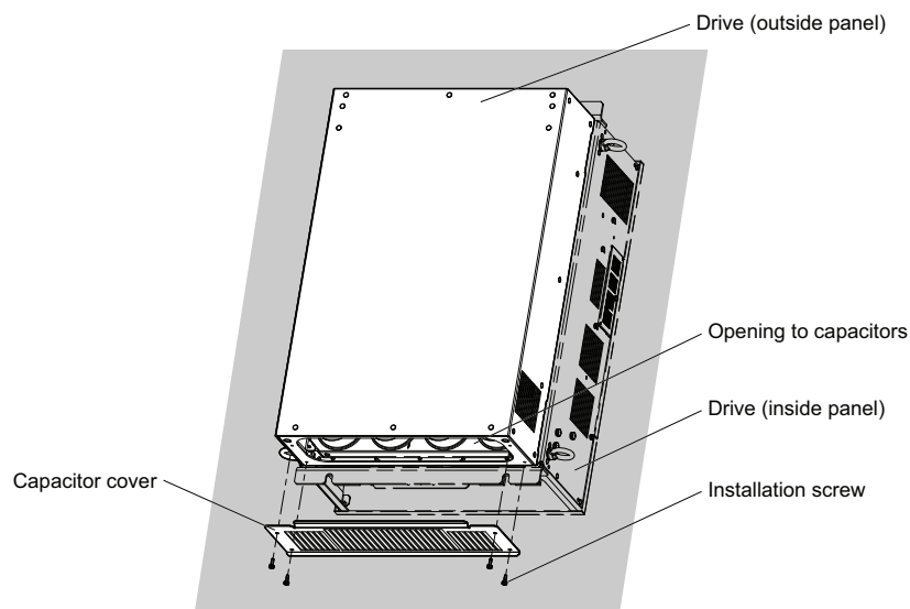
Figure 127 Capacitor Cover
