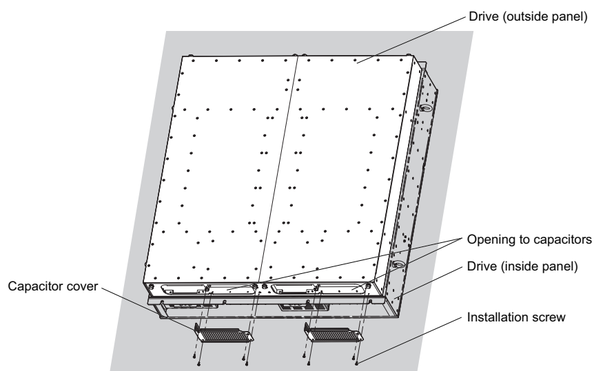
Figure 128 Capacitor Cover (4A0810, 4A1090)
