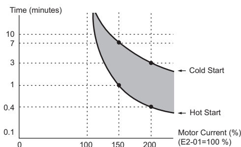
Motor Overload Protection Time
