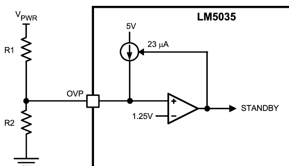
FIGURE 11. Basic Over-Voltage Protection
