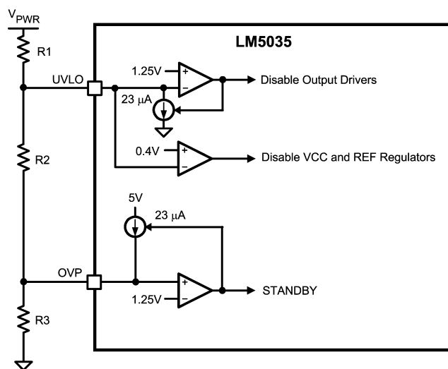
FIGURE 12. UVLO/OVP Divider
