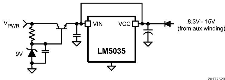
FIGURE 7. Start-up Regulator for V_{PWR} > 100V
