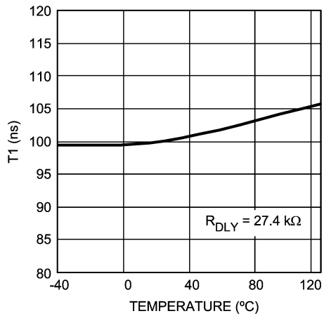
SR "T1" Parameter vs Temperature
