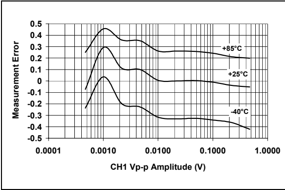
图 2-10: 测量误差, 增益 = 2, PF = + 0.5
