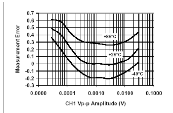
图 2-5: 测量误差, 增益 = 16, PF = +0.5
