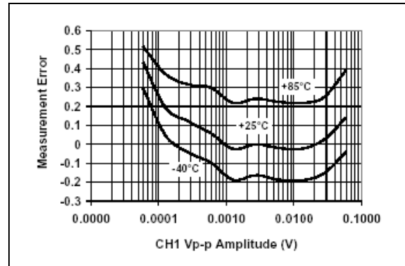
图 2-4: 测量误差, 增益 = 8, PF = +0.5
