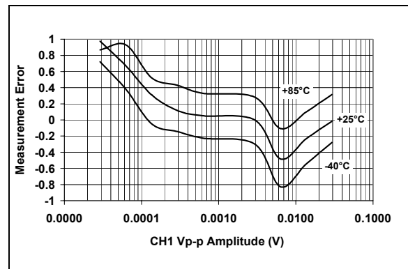
图 2-6: 测量误差, 增益 = 32, PF = +0.5
