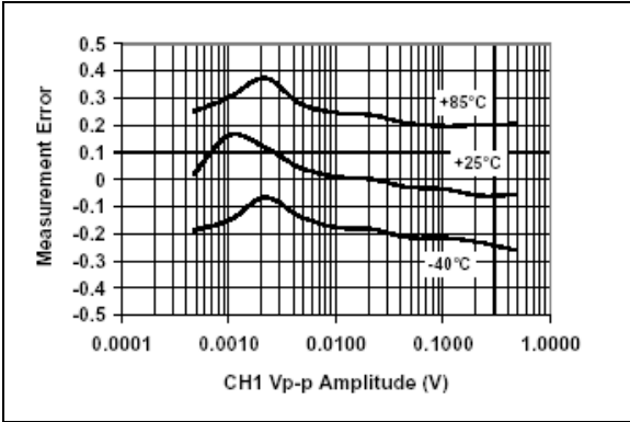
图 2-9: 测量误差, 增益 = 1, PF = + 0.5
