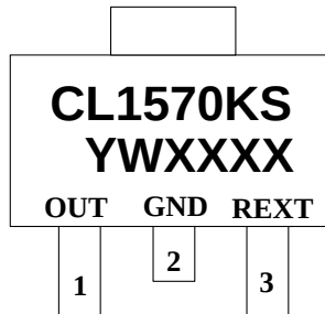
TO-252-2L
