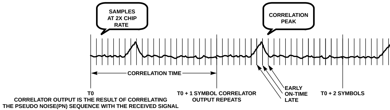
FIGURE 18. CORRELATION PROCESS
