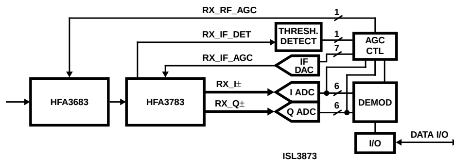
FIGURE 12. AGC CIRCUIT
