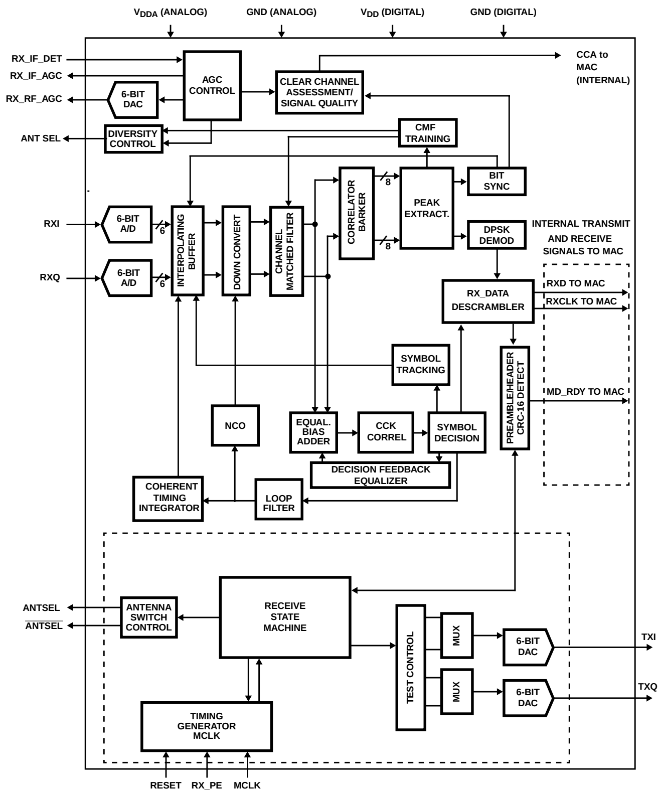
FIGURE 19. DSSS BASEBAND PROCESSOR, RECEIVE SECTION
