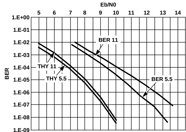
FIGURE 21. BER vs E_b/N_0 PERFORMANCE FOR CCK MODES
