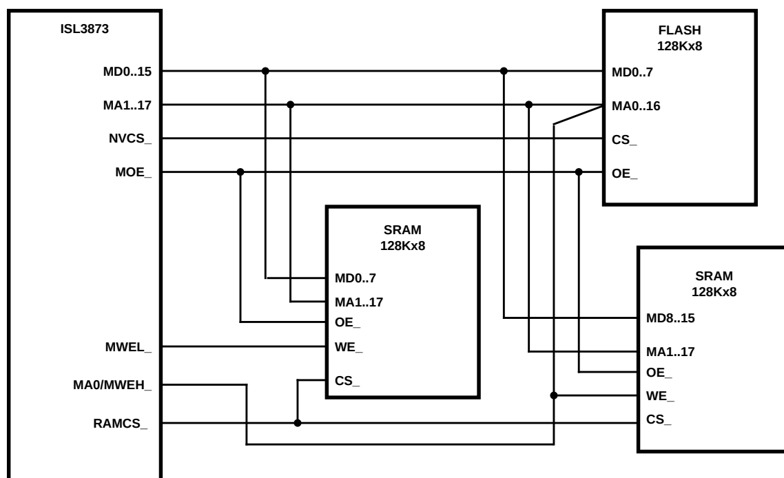
FIGURE 6. 8-BIT MEMORY INTERFACE REQUIREMENTS FOR ISL3873
