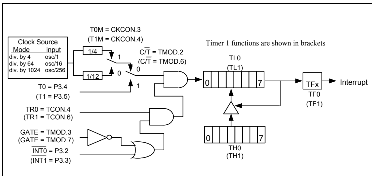
Figure 12. Timer/Counter Mode 2.
