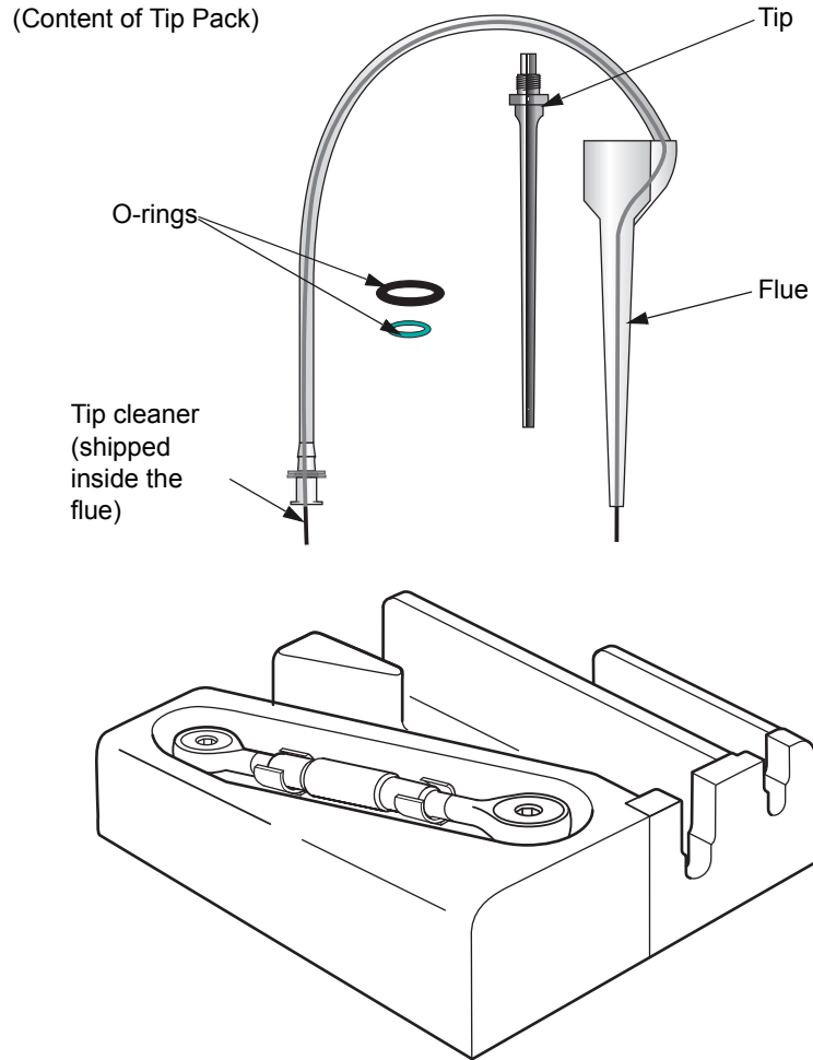
Figure 8-2 Tip torquing base and torque wrench (for use in non-sterile field)
