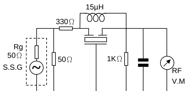
XT4.5MB TEST CIRCUIT
