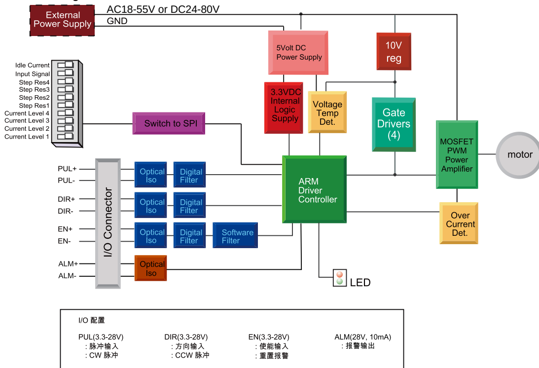
Block Diagram
