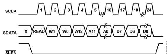
Figure 49. SPI Timing Diagram, Read Operation
