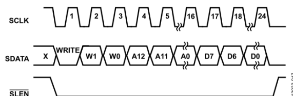
Figure 50. SPI Timing Diagram, Write Operation
