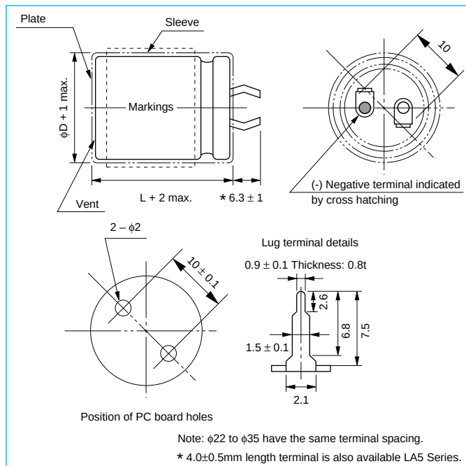
Outline Drawing
