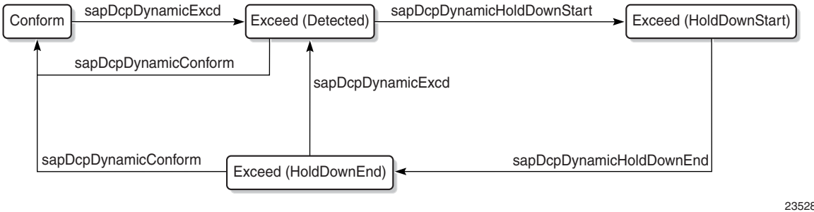
Figure 7 Dynamic policer alarm message sequence
