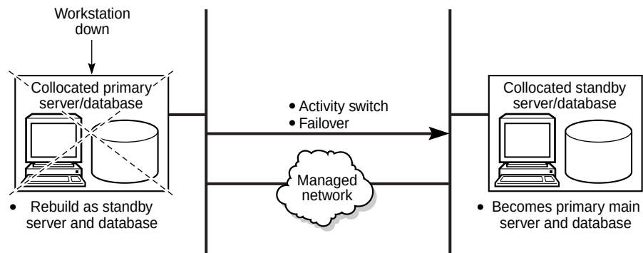
Figure 18 Primary server and database station down, collocated system
