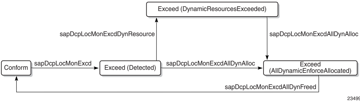
Figure 6 Local monitoring policer alarm message sequence
