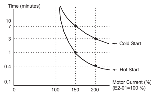
Figure 97 Motor Overload Protection Time
