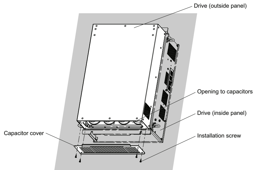
Figure 98 Capacitor Cover
