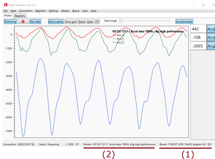
Figure 3. Example RoKiX Windows GUI software window
