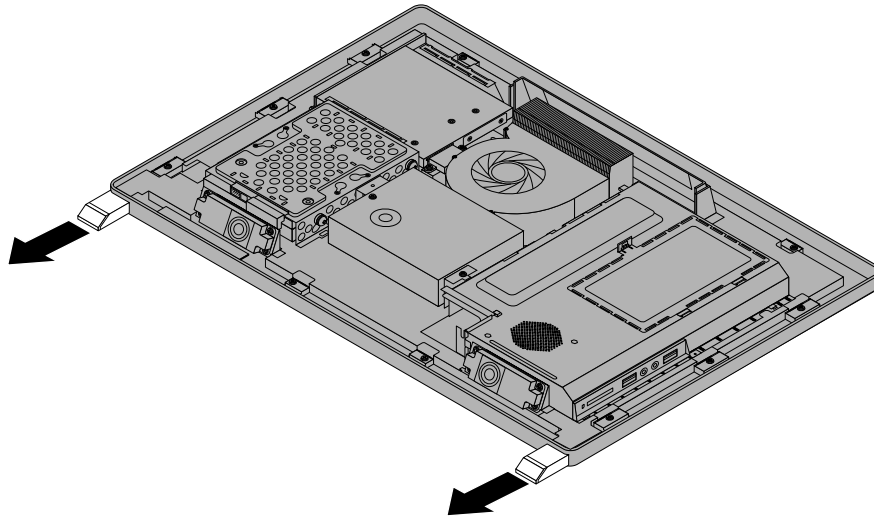
Figure 43. Removing the foot stands
