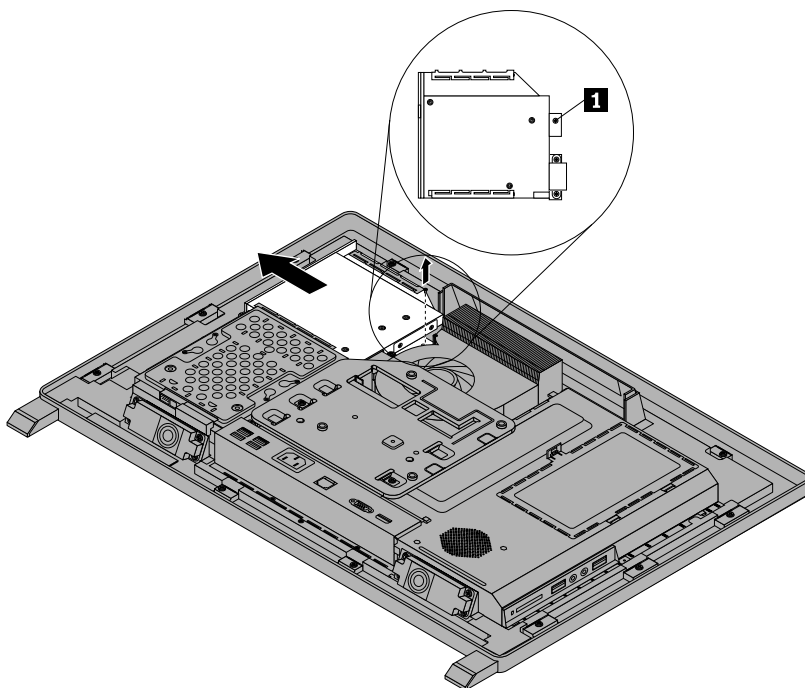
Figure 18. Removing the optical drive
