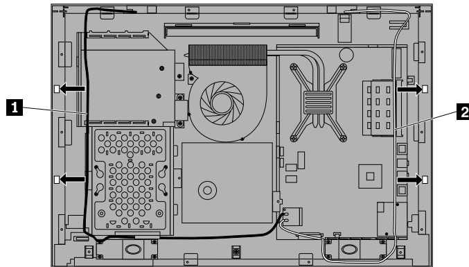
Figure 49. Replacing the wireless antenna wires
