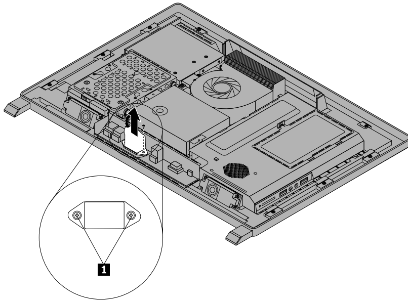
Figure 23. Removing the power cord connector
