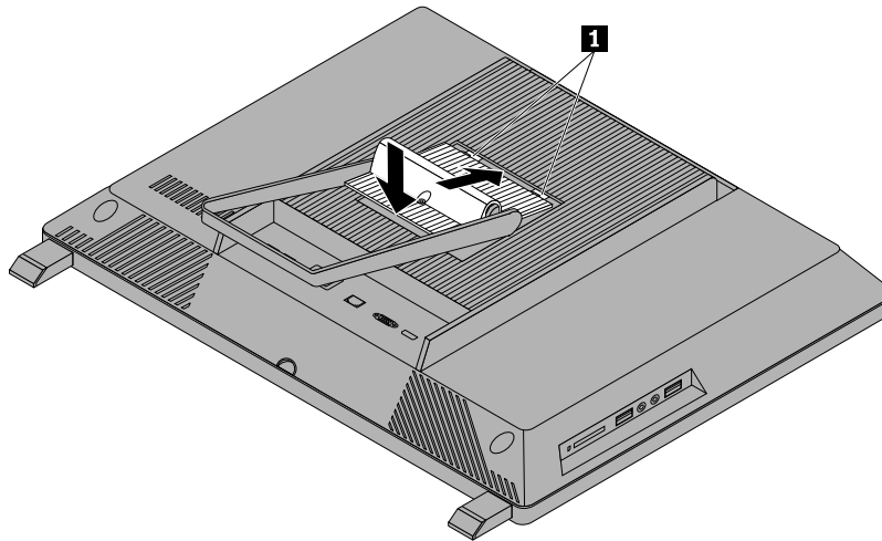
Figure 6. Reinstalling the system stand hinge cover
