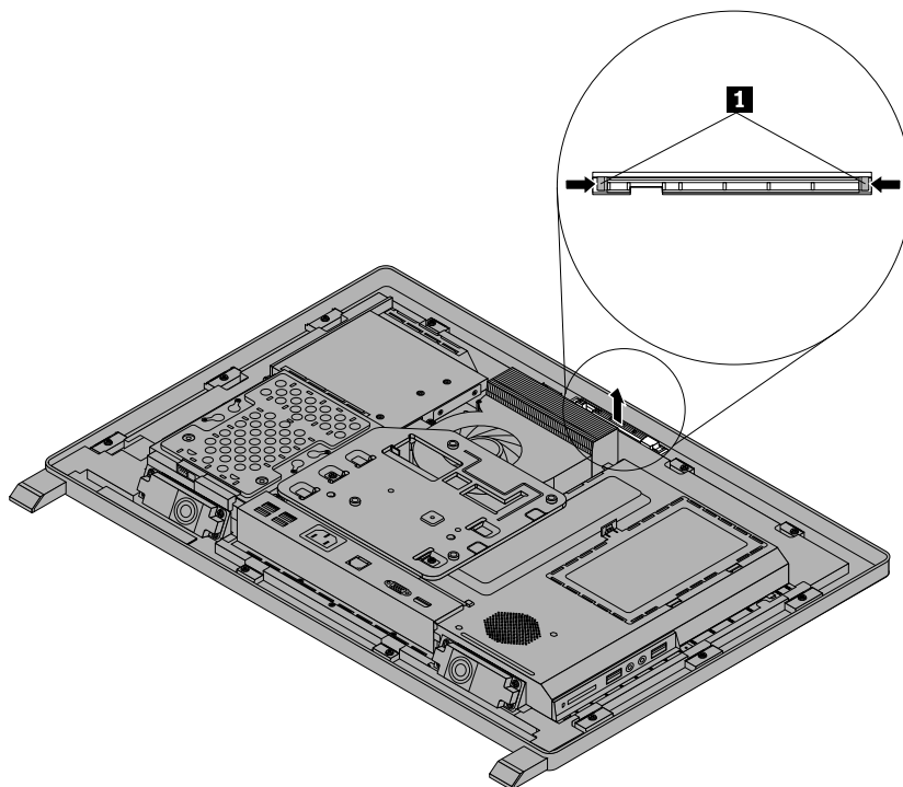
Figure 40. Removing the integrated camera
