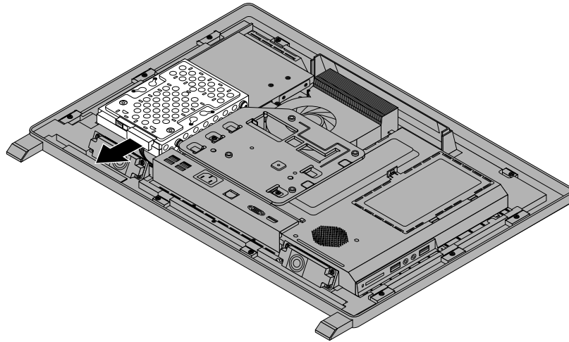
Figure 16. Removing the hard disk drive
