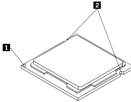
Figure 30. Noting the orientation of the microprocessor in the socket
