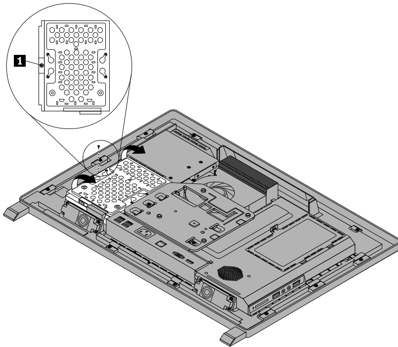
Figure 15. Removing the screw that secures the hard disk drive
