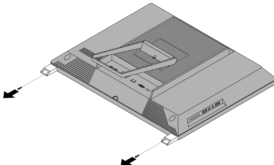
Figure 11. Removing each foot stand from the computer
