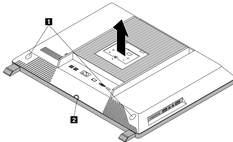
Figure 14. Removing the computer cover
