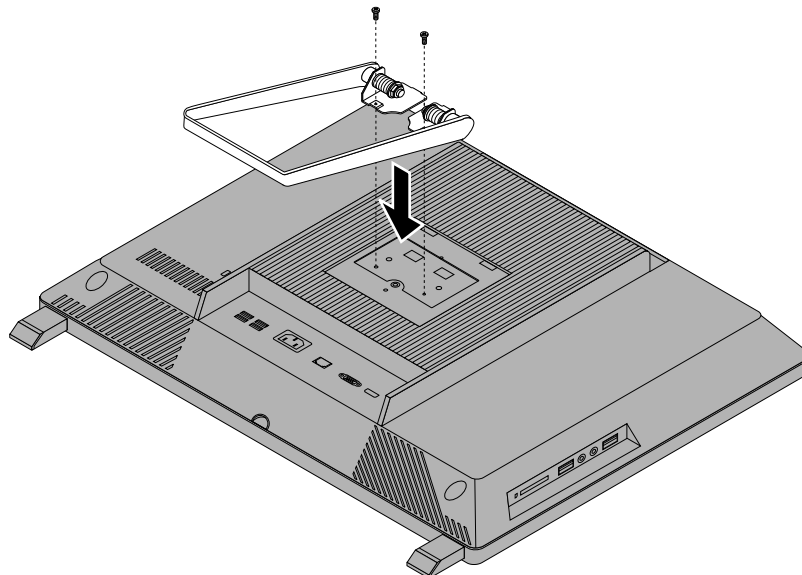
Figure 9. Reinstalling the system stand
