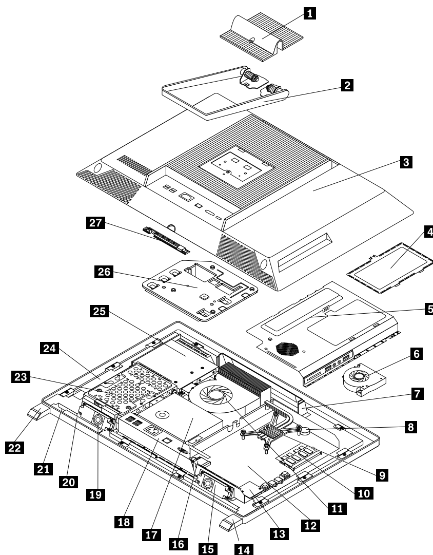
Figure 3. FRU locations
