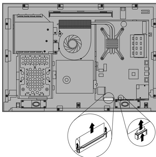
Figure 44. Disconnect the LCD panel cable and the touch panel control board cable from the system board
