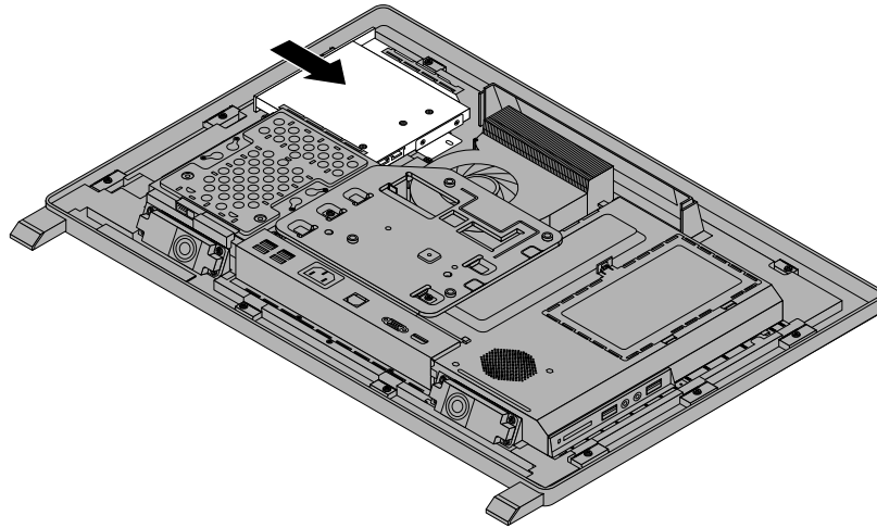
Figure 19. Installing the optical drive
