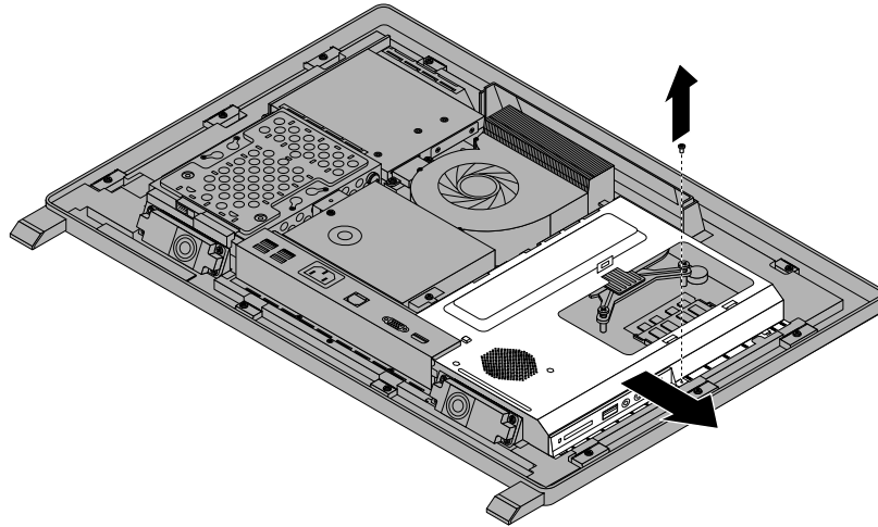
Figure 24. Removing the system board shield
