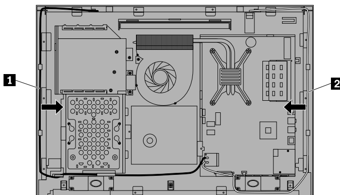
Figure 46. Loosening the wireless antenna wires from the computer main bracket
