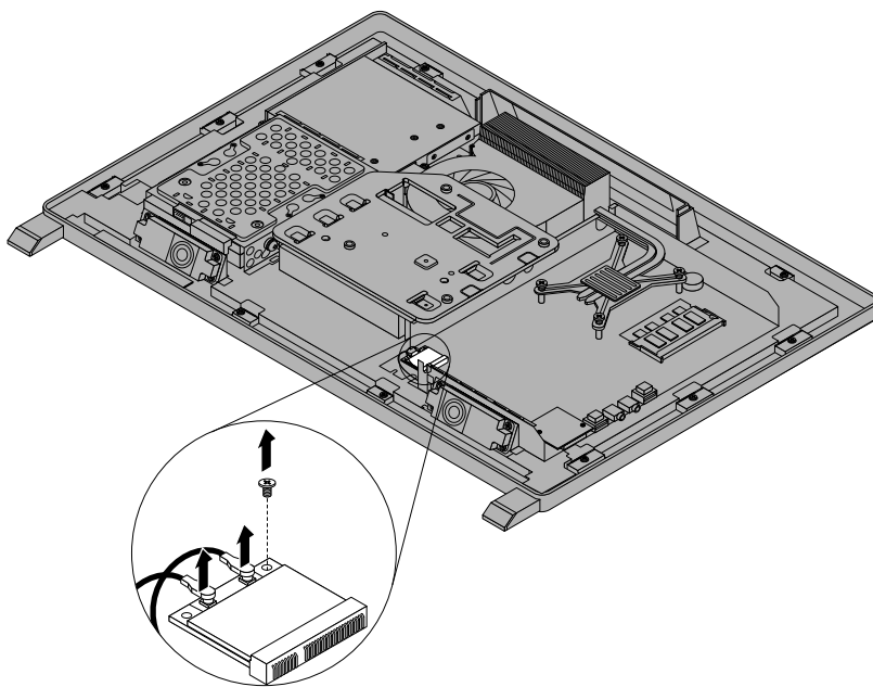
Figure 51. Removing the screw that secures the WI-FI card to the system board
