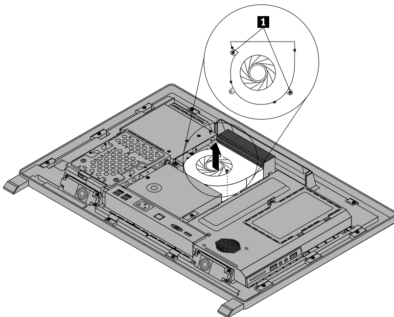
Figure 27. Removing the microprocessor fan
