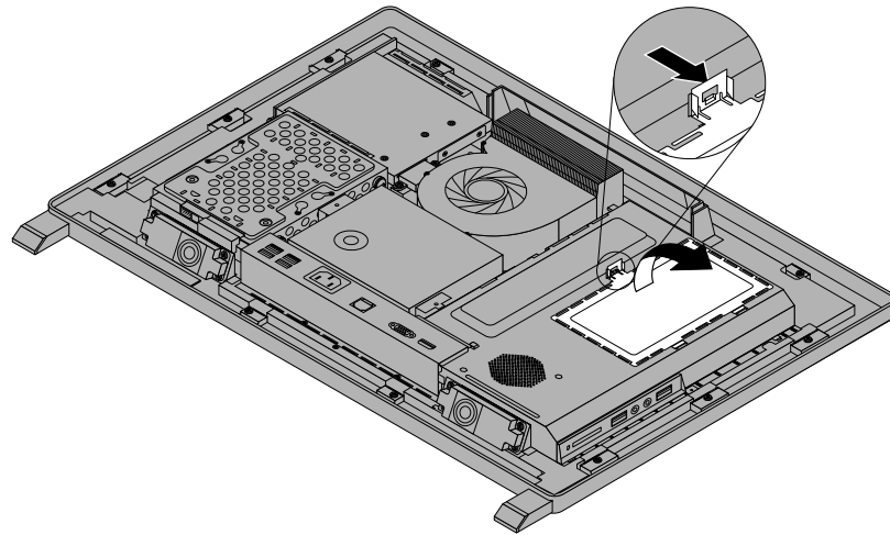
Figure 34. Opening the system board shield window
