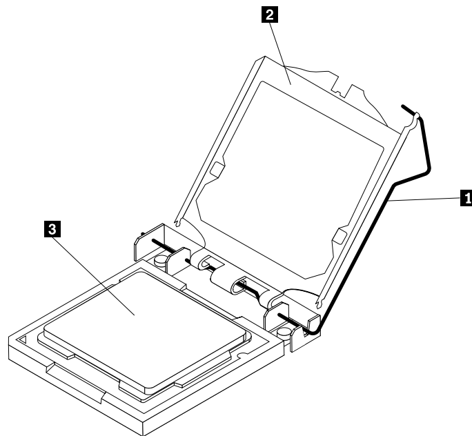
Figure 29. Opening the retainer to access the microprocessor
