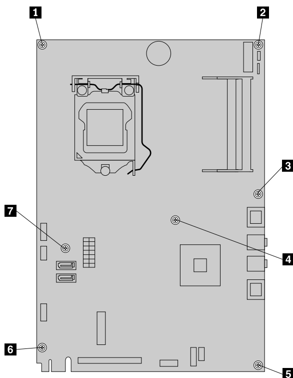
Figure 41. Removing the seven screws that secure the system board to the main bracket
