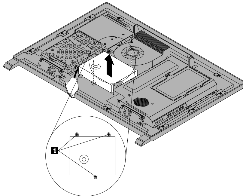
Figure 26. Removing the three screws that secure the power supply
