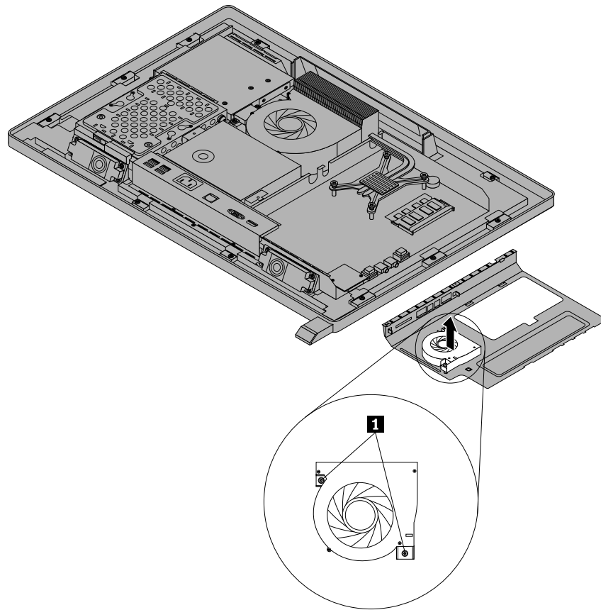
Figure 25. Removing the system fan
