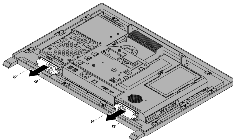
Figure 39. Removing the internal speakers
