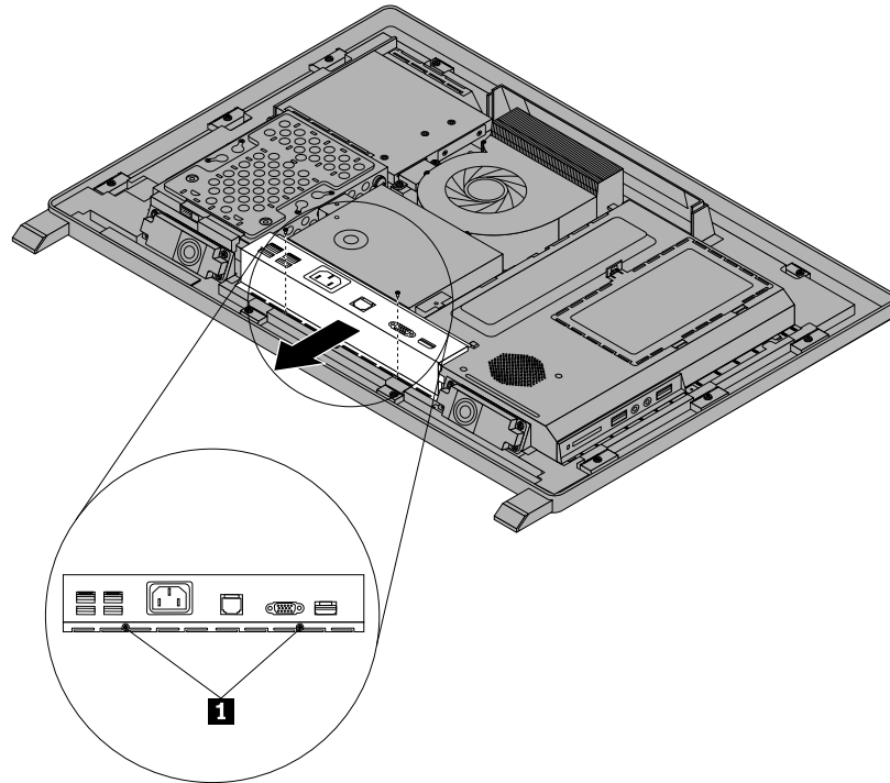
Figure 22. Removing the two screws that secure the rear I/O assembly
