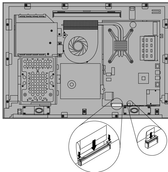
Figure 50. Reconnecting the LCD panel cable and the touch panel control board cable to the system board
