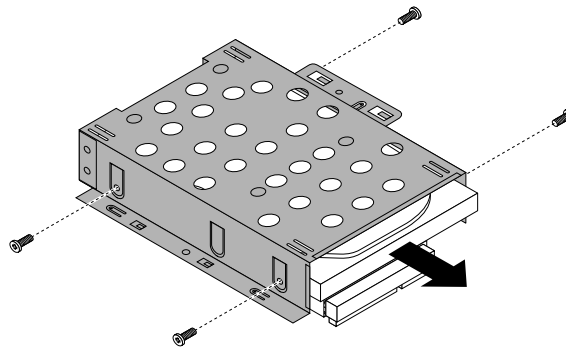
Figure 17. Removing the hard disk drive out of the bracket
