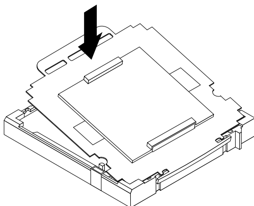
Figure 42. Installing one side of the socket cover into the microprocessor socket
