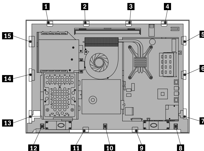
Figure 48. Reinstalling all the 15 screws that secure the computer main bracket to the front bezel
