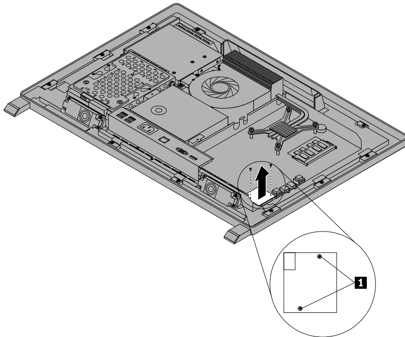
Figure 33. Removing the card reader
