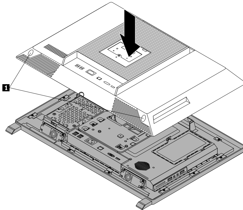
Figure 53. Installing the computer cover
