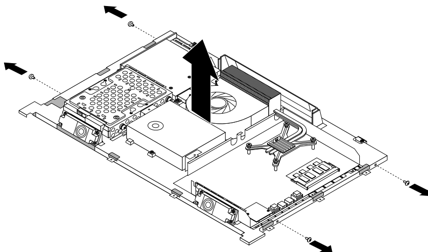
Figure 47. Removing the four screws that secure the LCD panel
