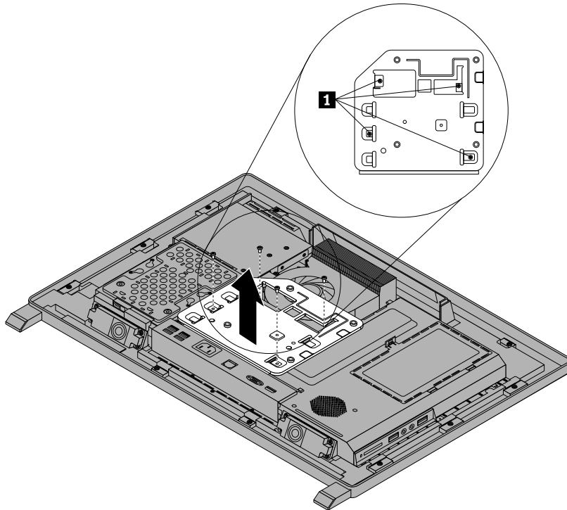
Figure 21. Removing the VESA mount bracket
