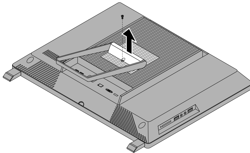
Figure 5. Removing the system stand hinge cover
