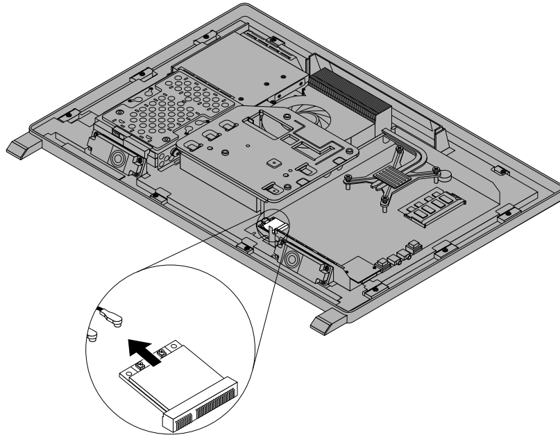
Figure 52. Removing the WI-FI card
