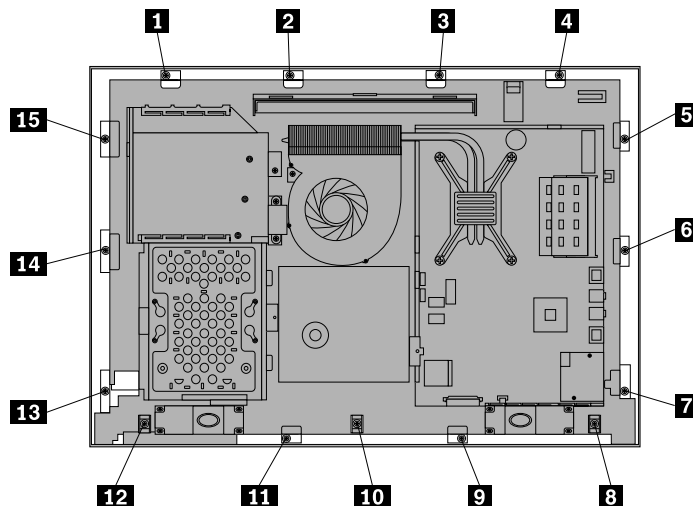
Figure 45. Removing all the 15 screws that secure the computer main bracket to the front bezel
