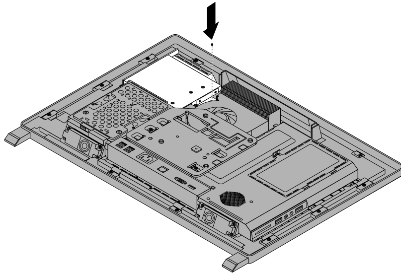
Figure 20. Installing the screw to secure the optical drive
