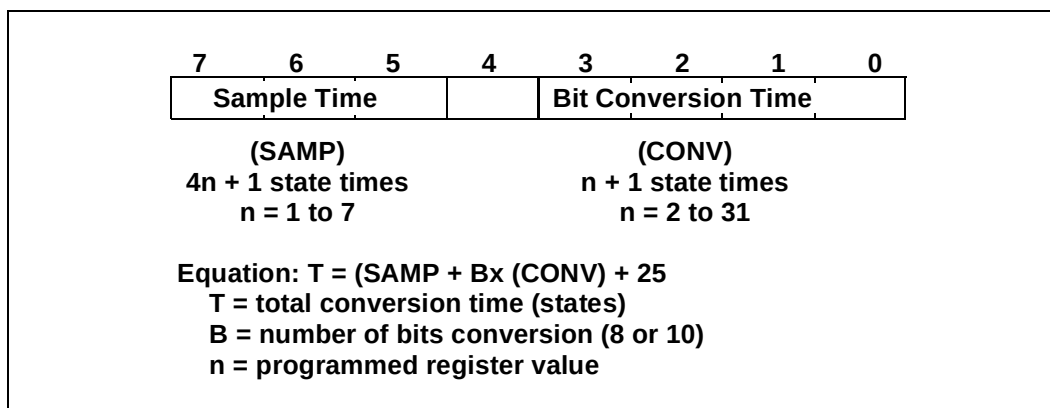
Figure 22. AD_TIME 1FAFH:Byte
