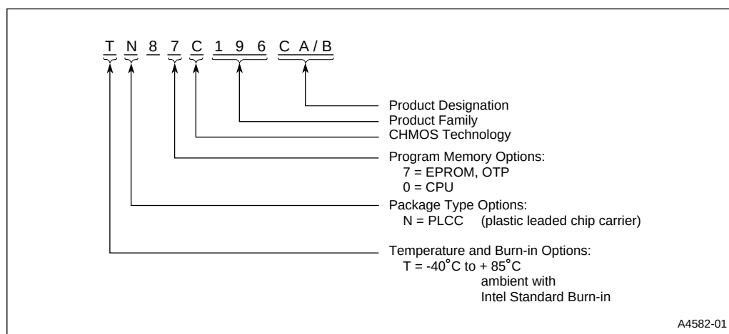
Figure 2. The 87C196CA/87C196CB - Express Family Nomenclature
