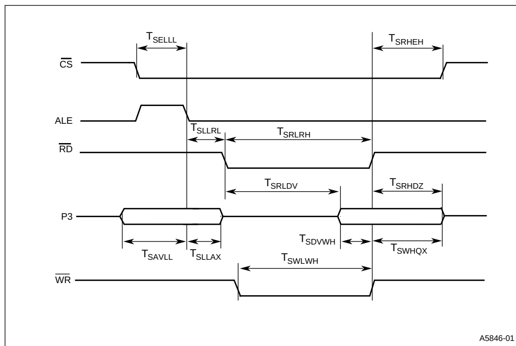
Figure 13. Slave Port Waveform - (SLPL = 1)
