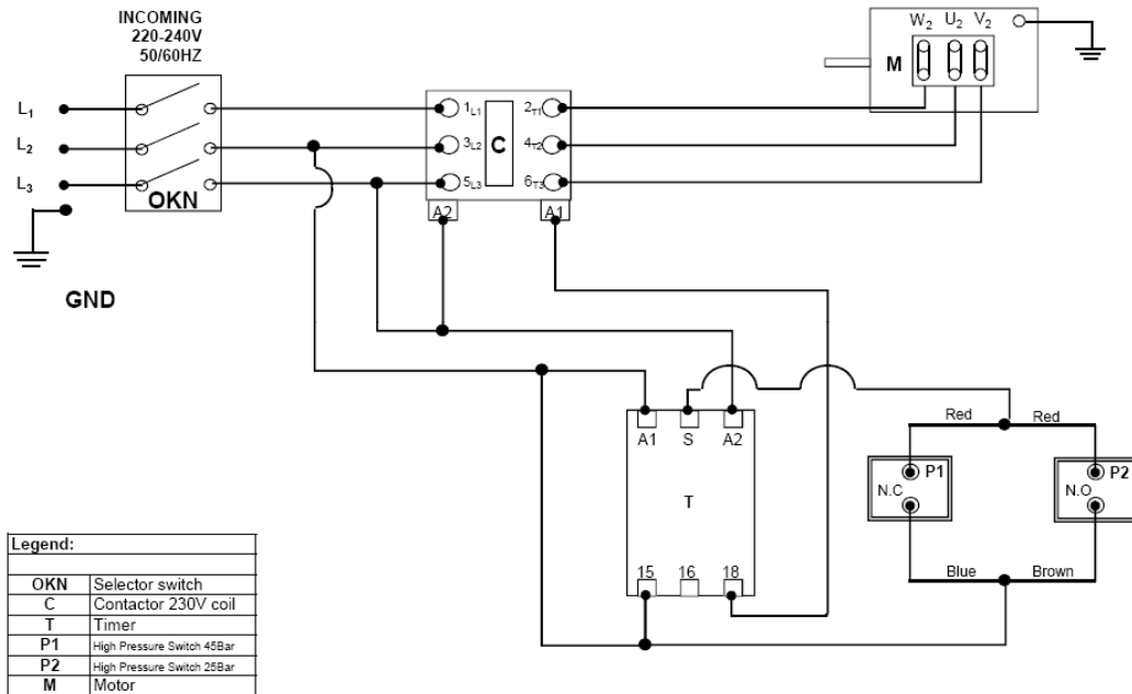
C-170/ 200 220-240V Three Phase with AUTO START STOP
