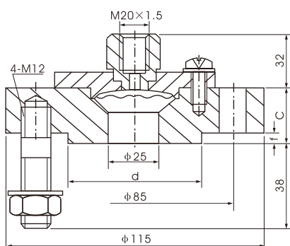
图三：MF型 ( P \leq 4\text{MPa} ) Drawing 3, MF Type
