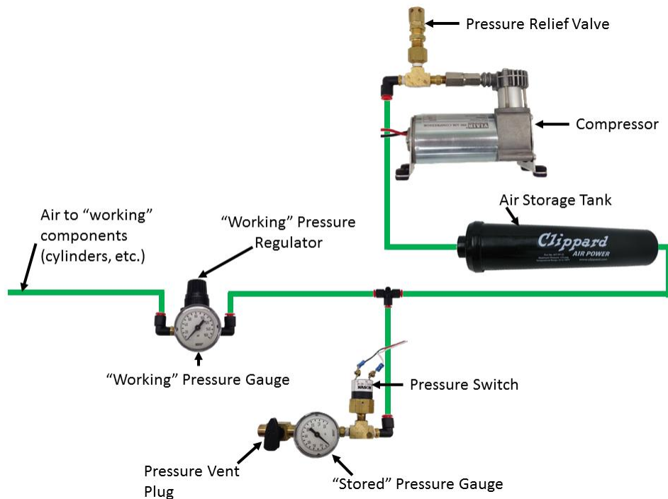
Figure 9-15 Pneumatic circuitry
