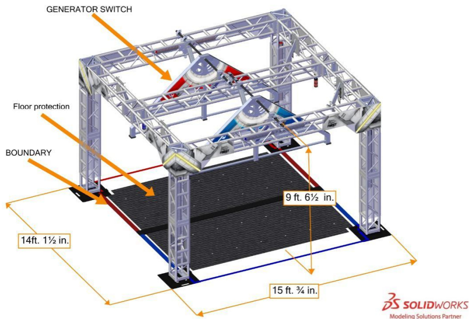
Figure 3-6 SHIELD GENERATOR
