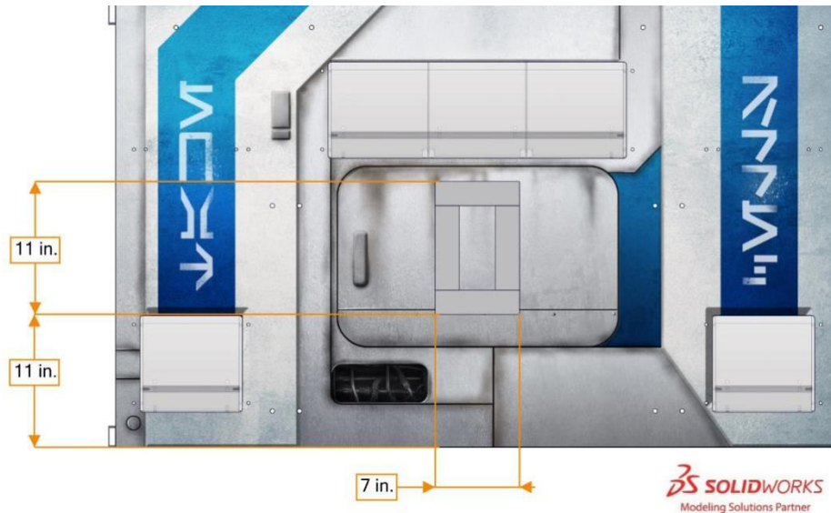
Figure 3-27 LOADING BAY vision target
