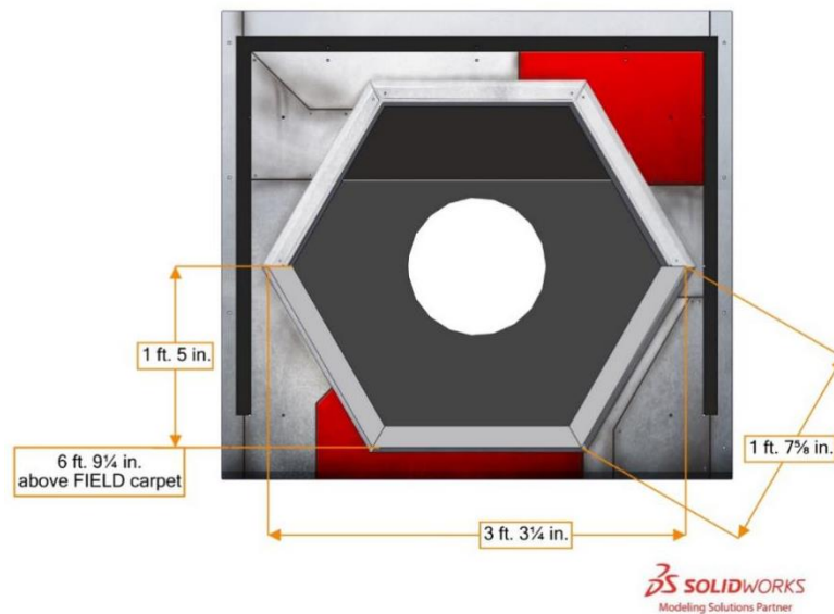
Figure 3-26 POWER PORT vision target
