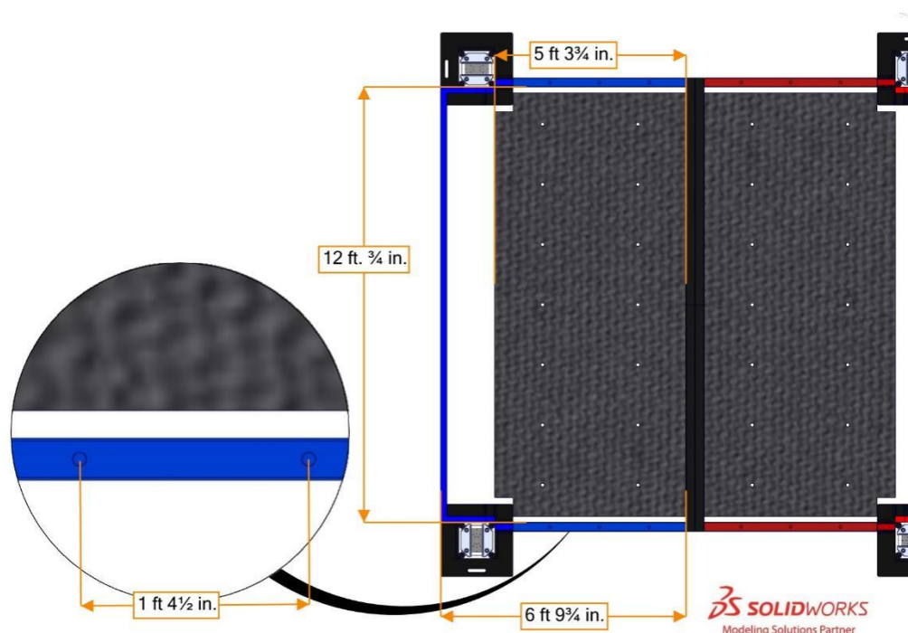
Figure 3-10 BOUNDARY dimensions
