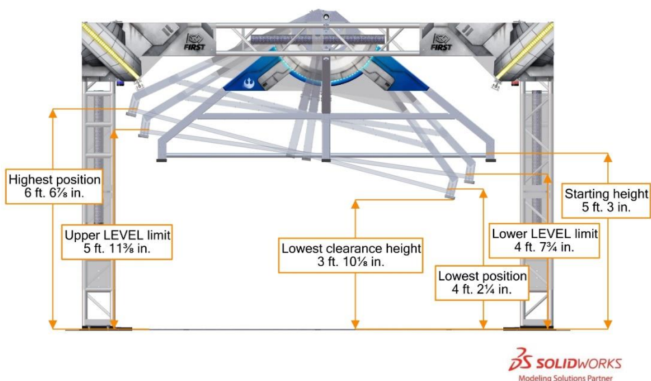
Figure 3-9 GENERATOR SWITCH range of motion (note: dimensions are to the top of the floor protection carpet)
