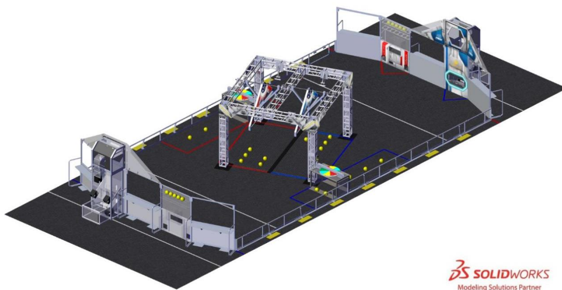
Figure 3-1 INFINITE RECHARGE
