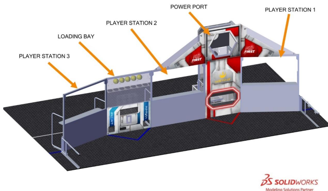
Figure 3-12 ALLIANCE WALL
