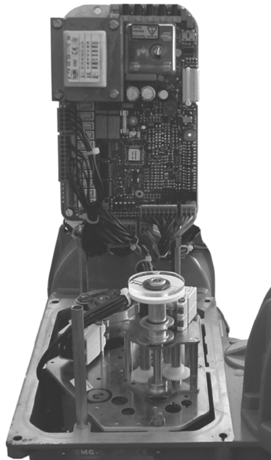
DPMC 30...119
