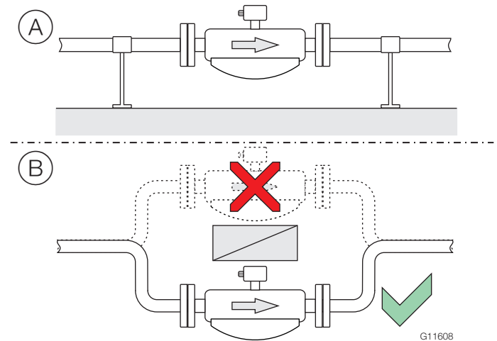
Fig. 5 Horizontal installation
