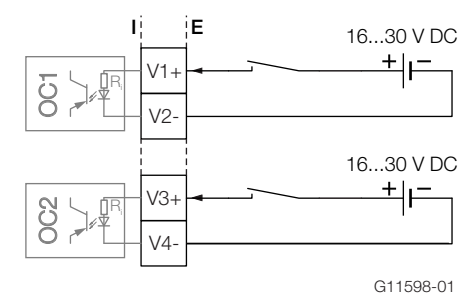
Fig. 38: Plug-in card as digital input (I = internal, E = external)
