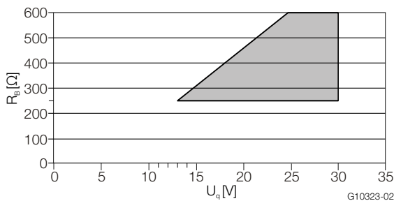
Fig. 33: Source voltage for passive outputs
