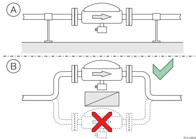
Fig. 6 Horizontal installation
