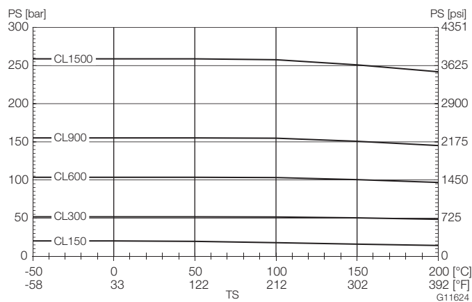
Fig. 15: Nickel alloy ASME flange C4 (2.4610) or nickel alloy C22 (2.4602) up to DN 200 (8 inch)
