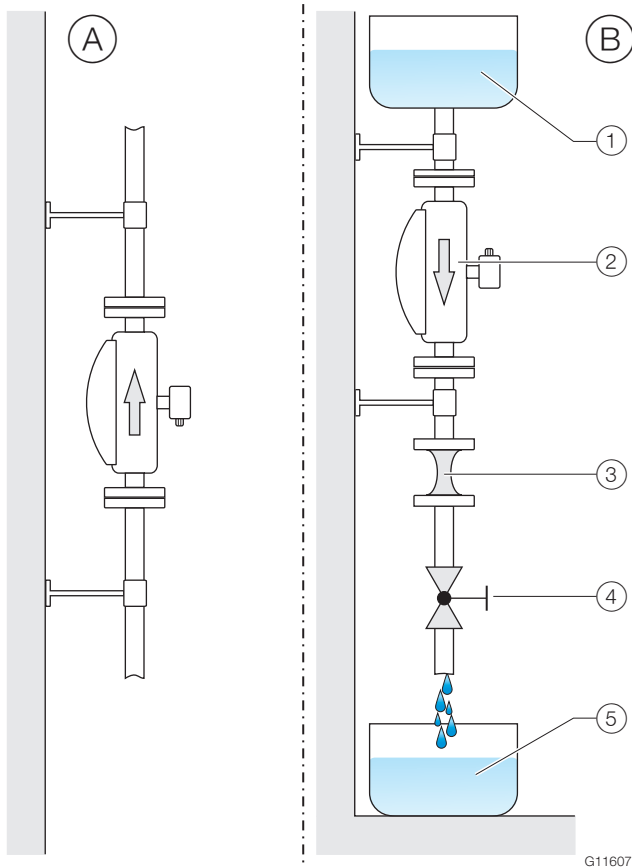
Fig. 4: Vertical installation
