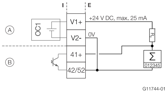
Fig. 40: Active digital output 41 / 42 (example)
