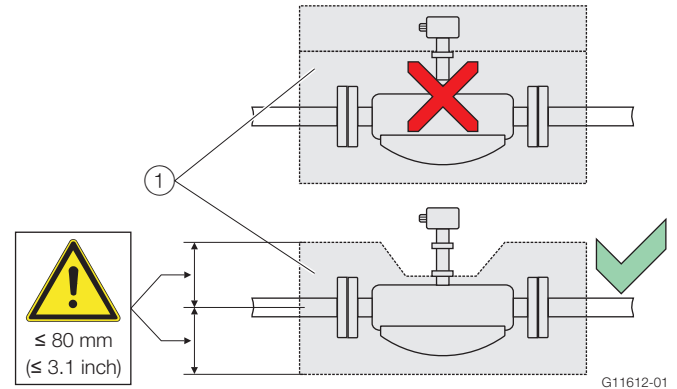
Fig. 7: Installation when T_{\text{medium}} is -50^{\circ}\text{C} \dots 205^{\circ}\text{C} ( -58 \dots 400^{\circ}\text{F} )
