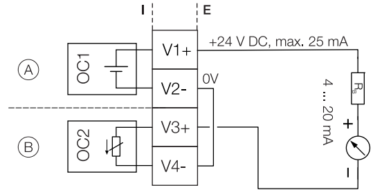
Fig. 42: Active current output V3 / V4 (example)
