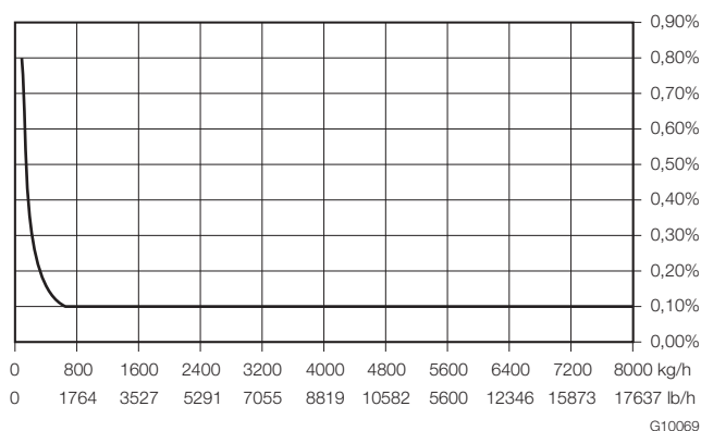
Fig. 10: Measured error FCB450 DN 15 (Example)
