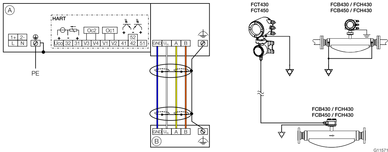
Fig. 31: (A) Transmitter (B) Sensor
