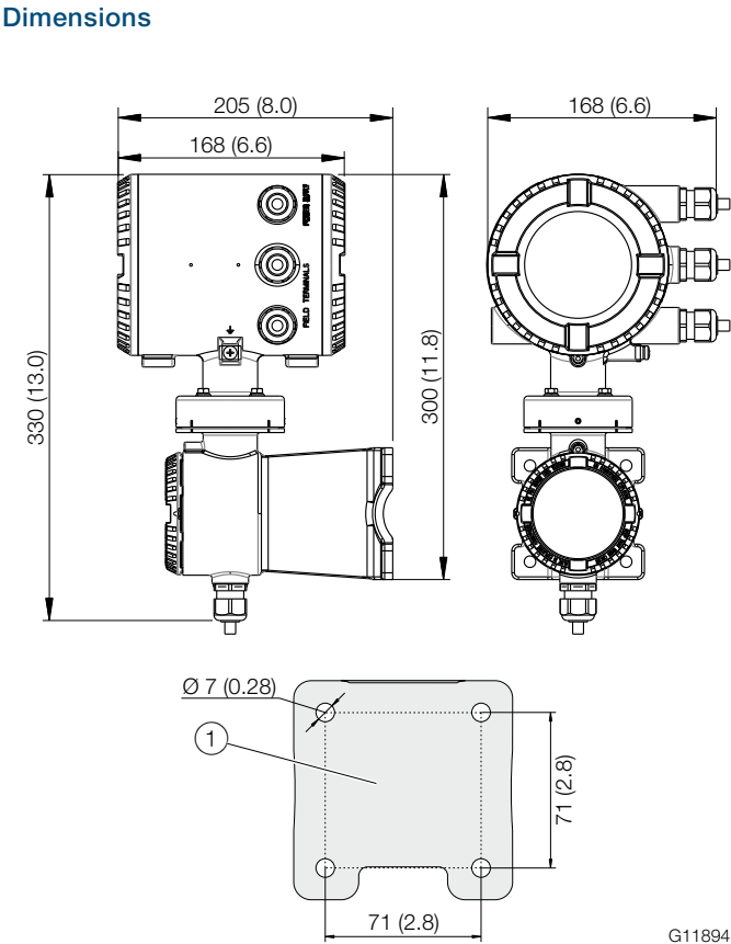
Fig. 44: Mounting dimensions of double-compartment housing
