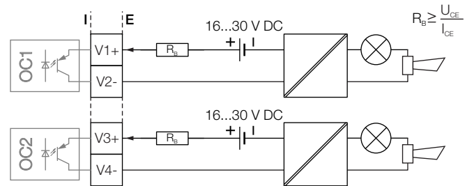
Fig. 37: Plug-in card as binary output (I = internal, E = external, R_B = load)
