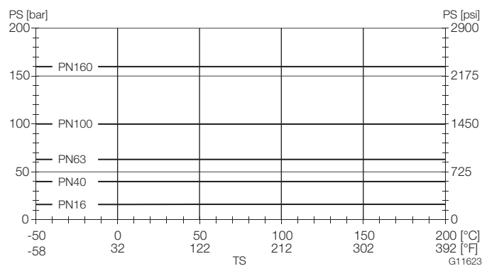
Fig. 14: Nickel alloy DIN flange C4 (2.4610) or nickel alloy C22 (2.4602) up to DN 200 (8 inch)
