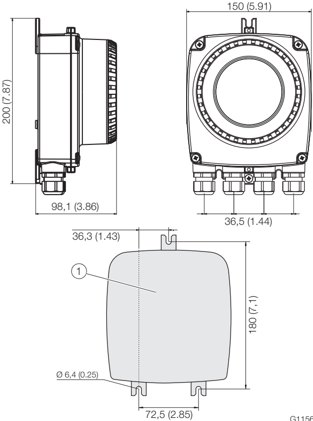
Fig. 45: Mounting dimensions single-compartment housing
