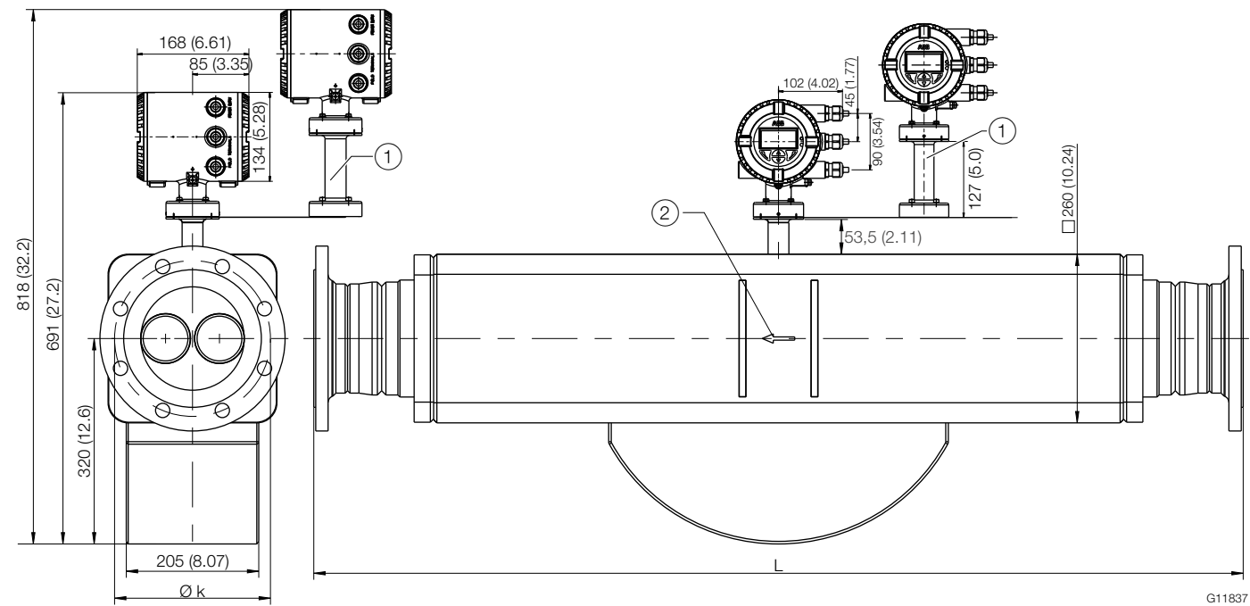
Fig. 19: Integral mount design with dual-compartment transmitter housing ① Option TE1 "Extended tower length" or option PR4 / PR5 / PR6 / PR7 "Pressure-resistant sensor housing" ② Flow direction
