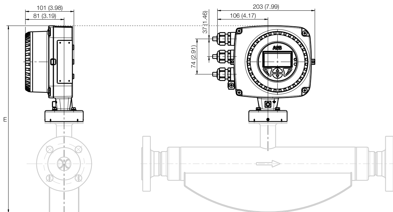
Fig. 28: Integral mount design with single-compartment transmitter housing
