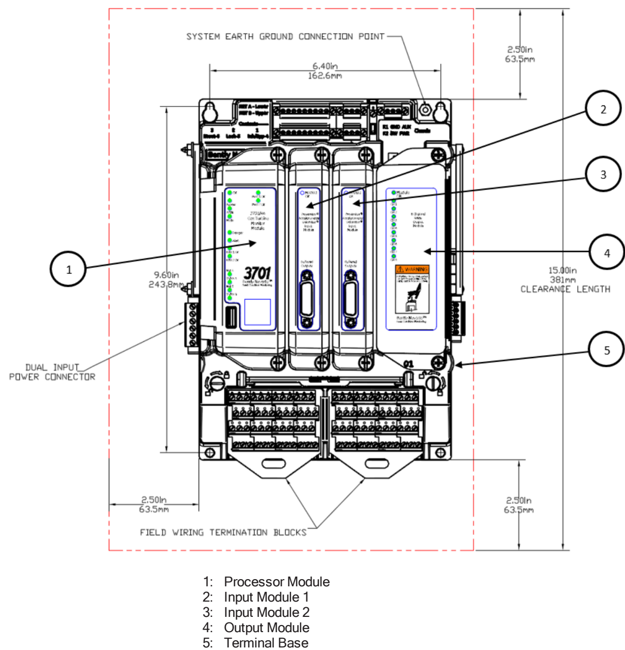
Figure 1: 3701/44 Simplex Terminal Base Top View
