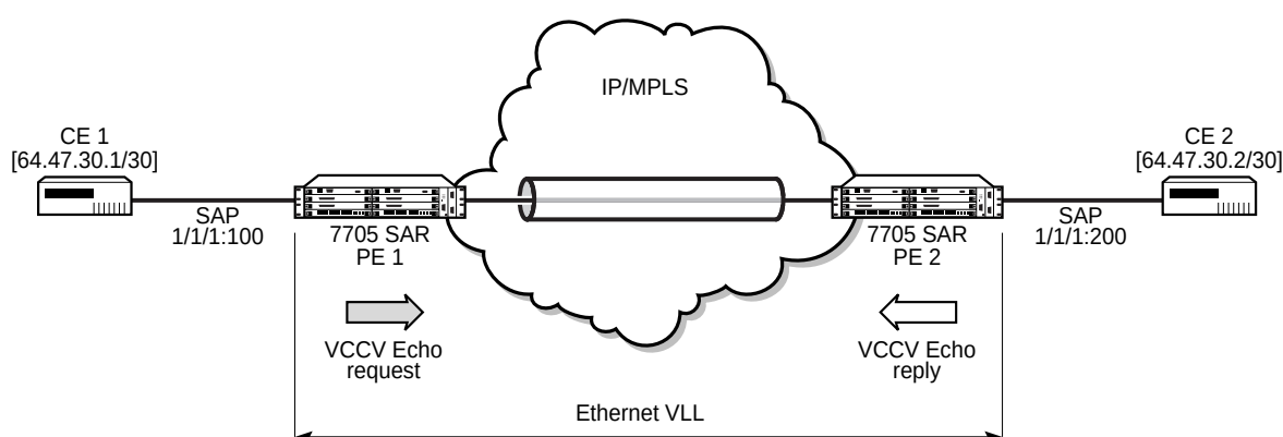
Figure 19: VCCV-Ping Application
