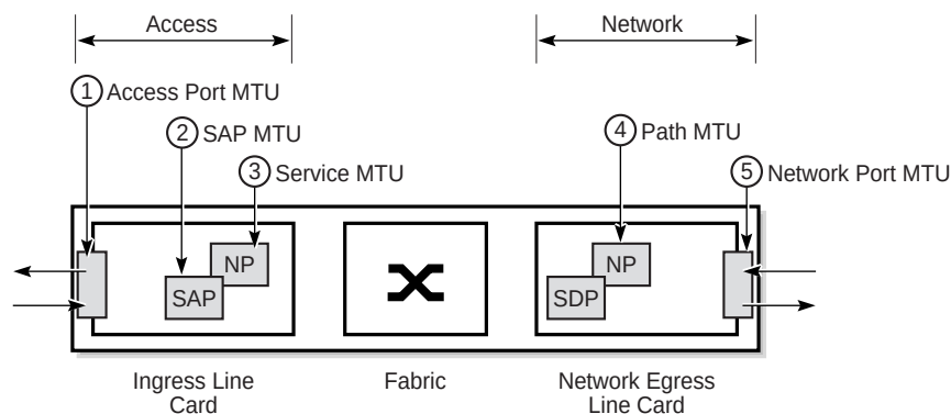
Figure 17: MTU Points on the 7705 SAR
