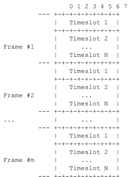
Figure 11: CESoPSN Packet Payload Format for Trunk-Specific N \times 64 kb/s
