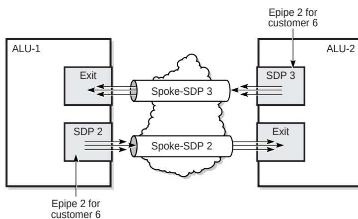
Figure 18: SDPs — Unidirectional Tunnels
