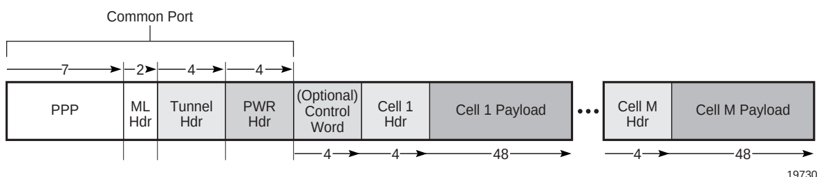
Figure 16: N-to-1 Cell Mode Encapsulation
