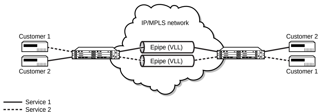
Figure 14: Epipe Service
