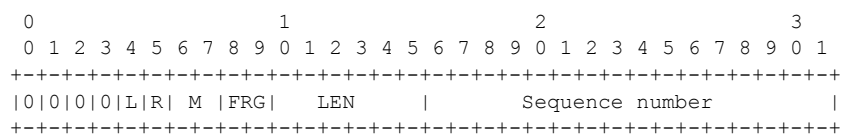
Figure 12: Control Word Bit Structure
