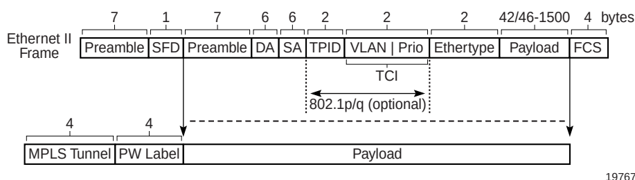
Figure 13: Ethernet VLL Frame with MPLS Encapsulation
