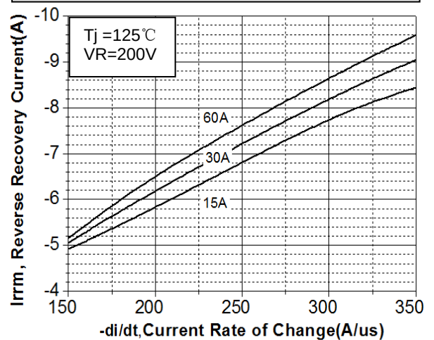
Fig.6 Peak reverse recovery current versus diF/dt
