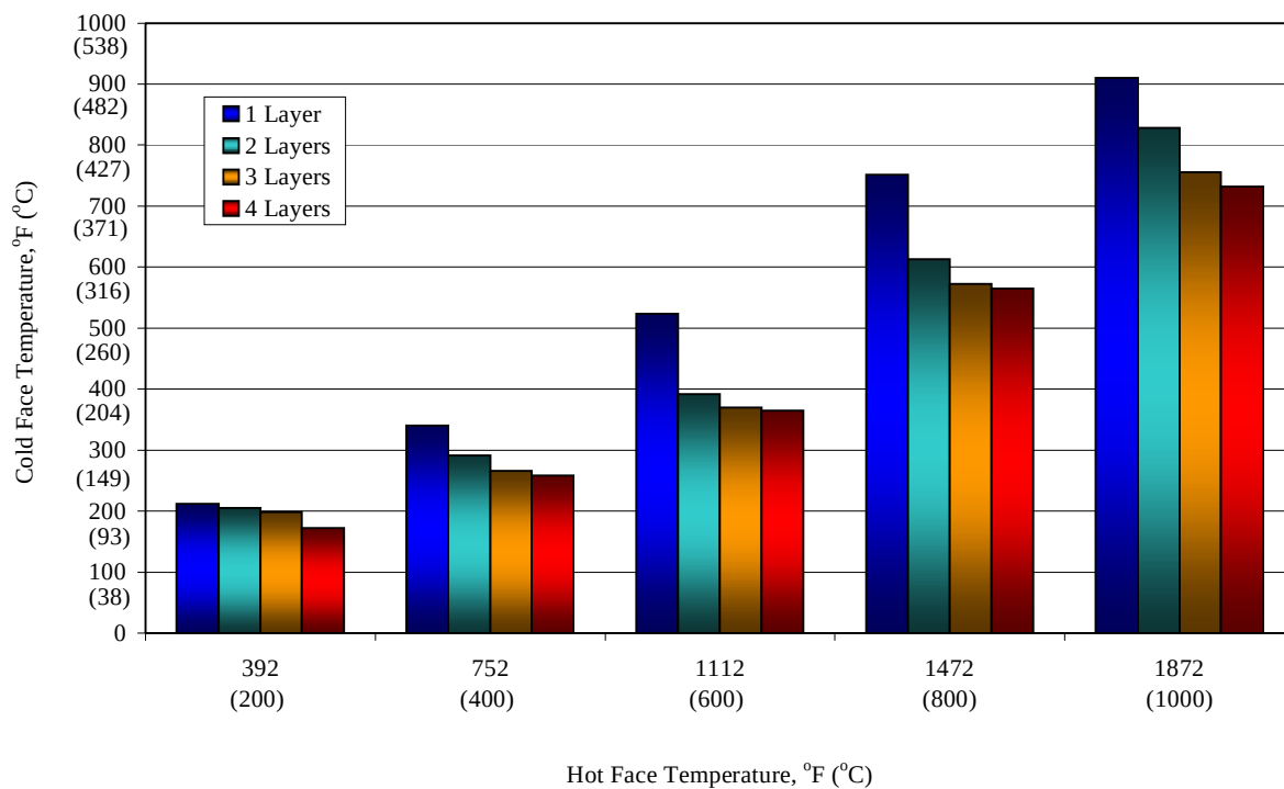
3M™ Nextel™ Woven Ceramic Fabric 440 Style BF-30 Hot Face vs. Cold Face
