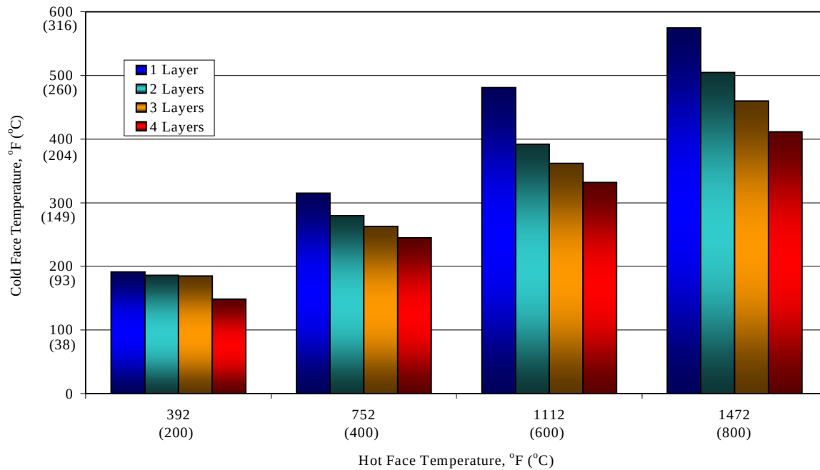
3M™ Nextel™ Woven Ceramic Fabric 440 Style BF-20 Hot Face vs. Cold Face
