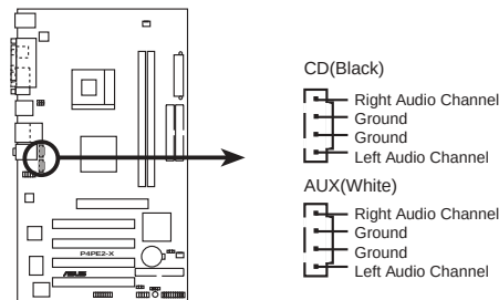
P4PE2-X Internal Audio Connectors
