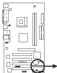
P4PE2-X Floppy Disk Drive Connector
