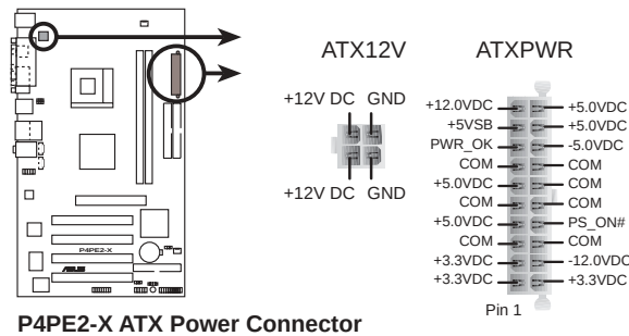
P4PE2-X ATX Power Connector
