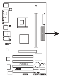
P4PE2-X IDE Connectors
