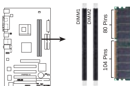
P4PE2-X 184-Pin DDR DIMM Sockets
