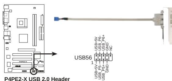
P4PE2-X USB 2.0 Header
