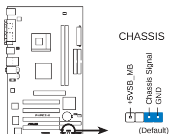
P4PE2-X Chassis Alarm Lead
