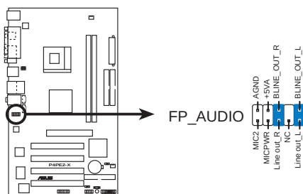
P4PE2-X Front Panel Audio Connector
