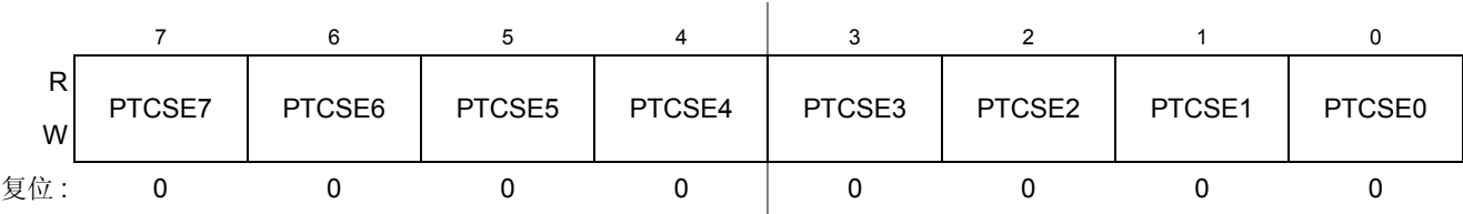
Figure 0-48. C 端口寄存器斜率使能 (PTCSE)
