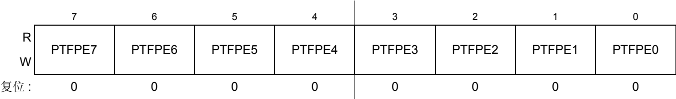
Figure 0-65. 端口寄存器内部上拉使能 (PTFPE)
