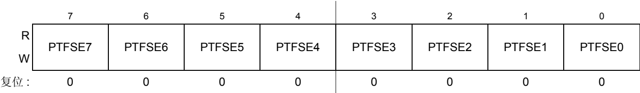
Figure 0-66. F 端口寄存器斜率使能 (PTFSE)
