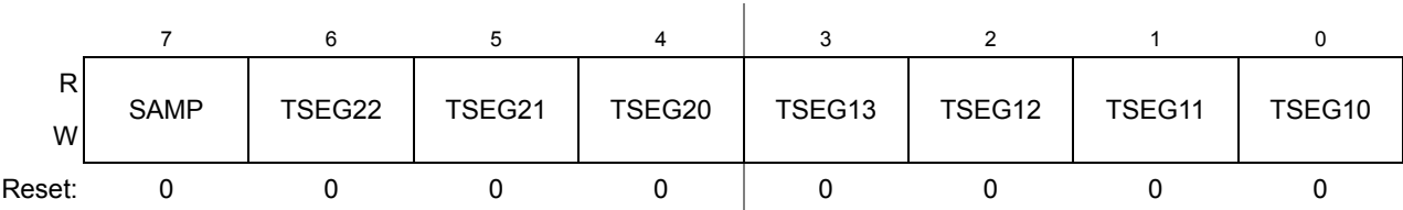
Figure 13-7. MSCAN 总线计时寄存器 1 (CANBTR1)
