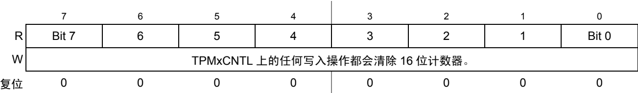
Figure 18-13. 定时器计数器寄存器低 (TPMxCNTL)
