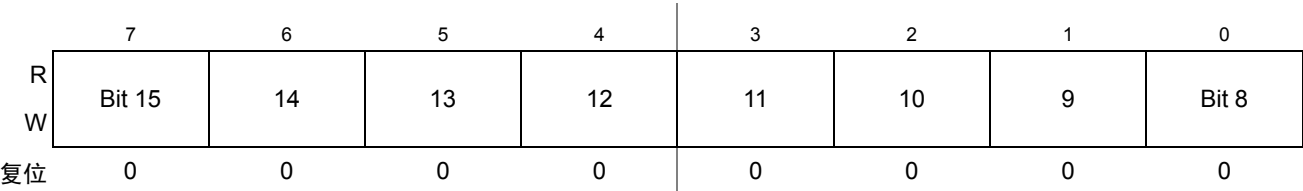
Figure 18-14. 定时器计数器模量寄存器高 (TPMxMODH)
