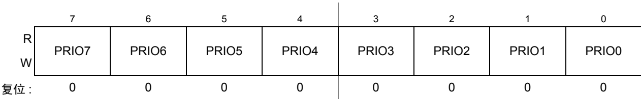
Figure 13-38. 发送缓冲器优先寄存器 (TBPR)
