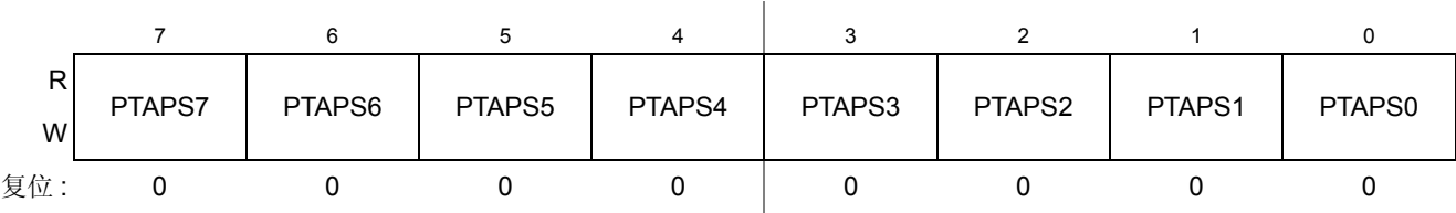
Figure 0-35. A 端口中断管脚选择寄存器 (PTAPS)
