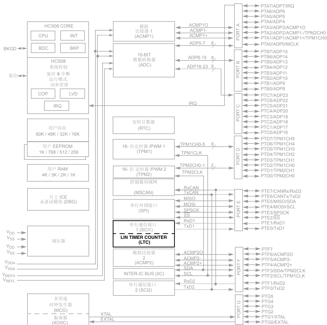
Figure 12-1. MC9S08DZ60/48/32/16 结构图，突显了 LTC 块和管脚
