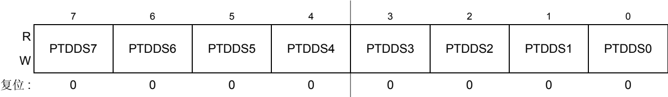
Figure 0-54. D 端口寄存器驱动强度选择 (PTDDS)
