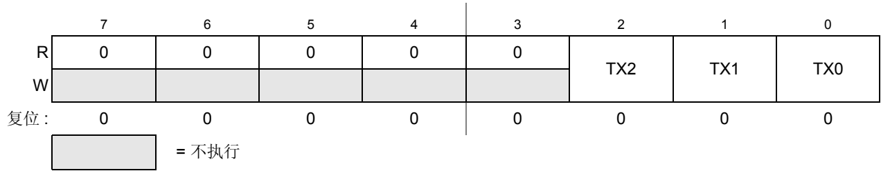
Figure 13-14. MSCAN 发送缓冲器选择寄存器 (CANTBSEL)
