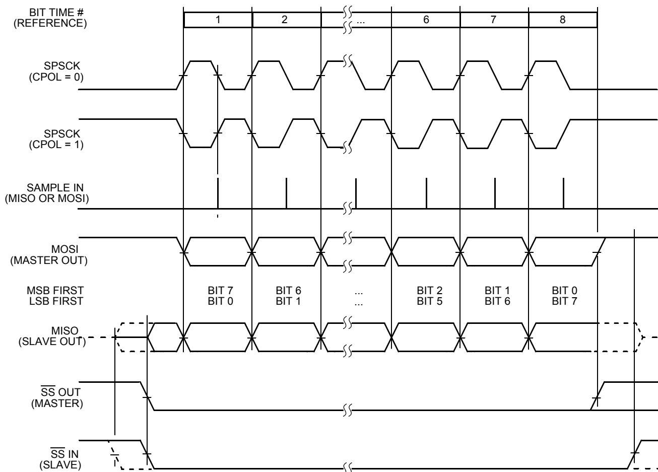
Figure 14-10. SPI 钟格式 (CPHA = 1)
