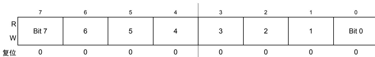
Figure 17-14. TPM 通道值寄存器低字节 (TPMxCnVL)
