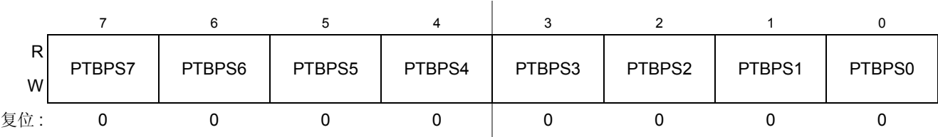
Figure 0-43. B 端口中断管脚选择寄存器 (PTBPS)
