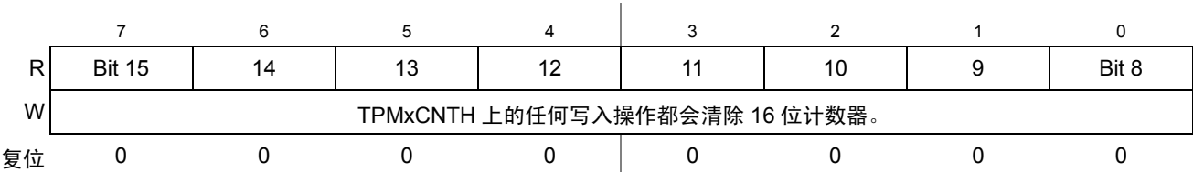
Figure 18-12. 定时器计数器寄存器高 (TPMxCNTH)
