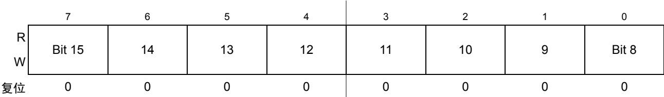
Figure 17-13. TPM 道值寄存器高字节 (TPMxCnVH)
