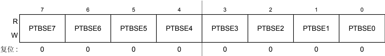
Figure 0-40. B 端口寄存器斜率使能 (PTBSE)
