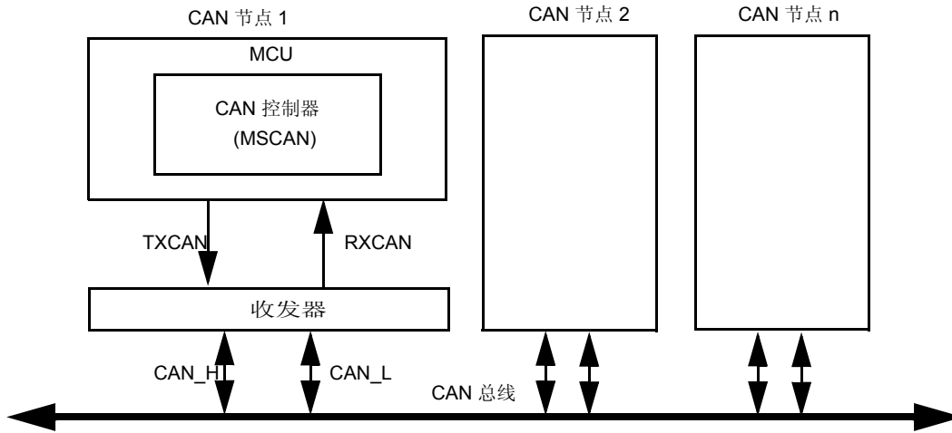
Figure 13-3. CAN System
