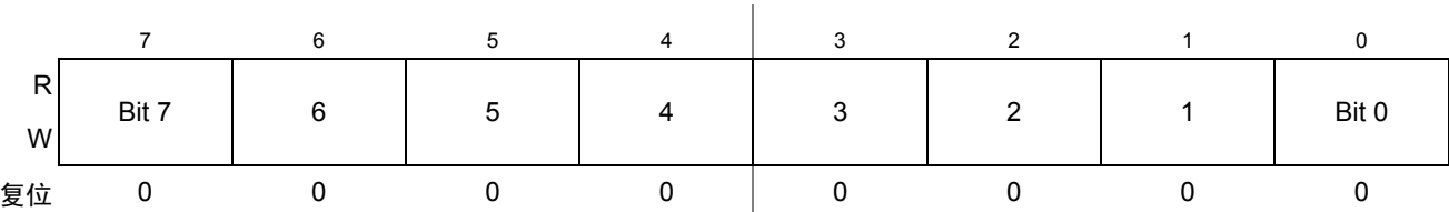
Figure 18-15. 定时器计数器模量寄存器低 (TPMxMODL)
