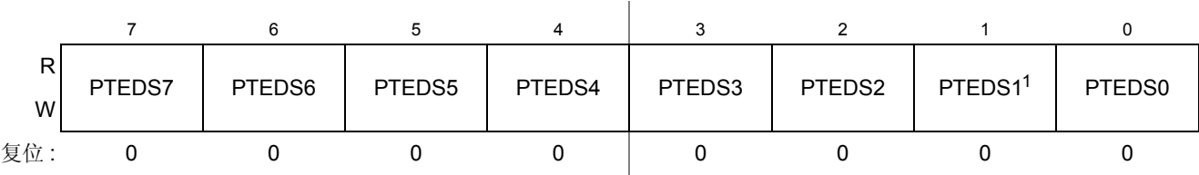
Figure 0-62. E 端口寄存器驱动强度选择 (PTEDS)
