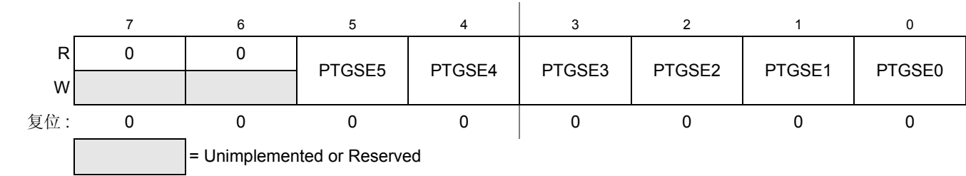
Figure 0-71. G 端口寄存器斜率使能 (PTGSE)
