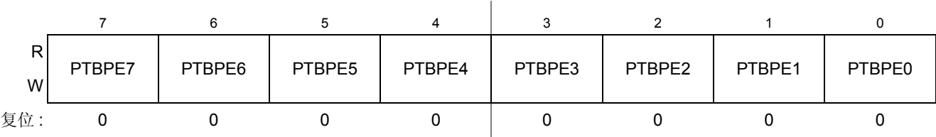
Figure 0-39. B 端口寄存器内部上拉使能 (PTBPE)
