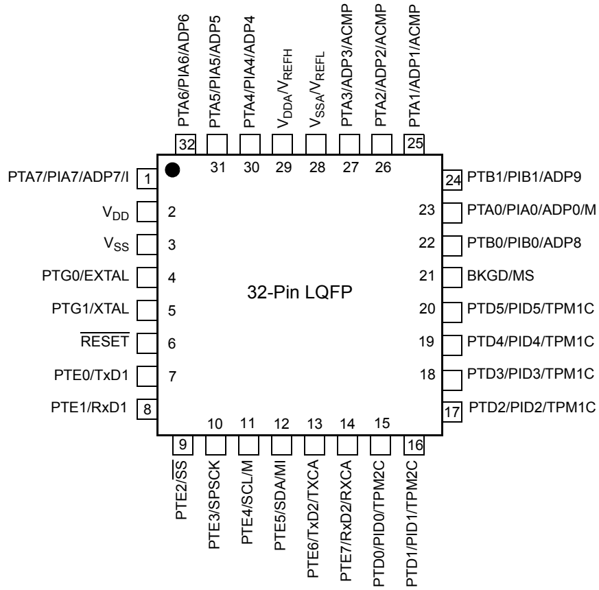
Figure 0-5. 32 管脚 LQFP
