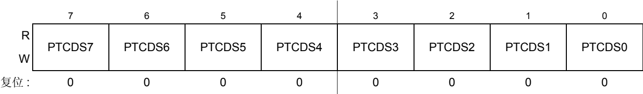
Figure 0-49. C 端口寄存器的驱动强度选择 (PTCDS)
