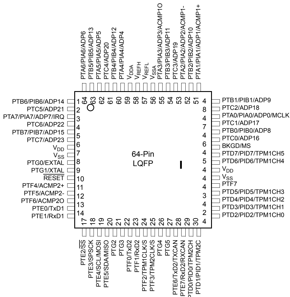
Figure 0-3. 64 管脚 LQFP
