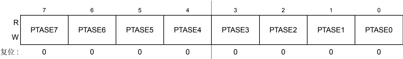
Figure 0-32. A 端口寄存器的斜率使能 (PTASE)
