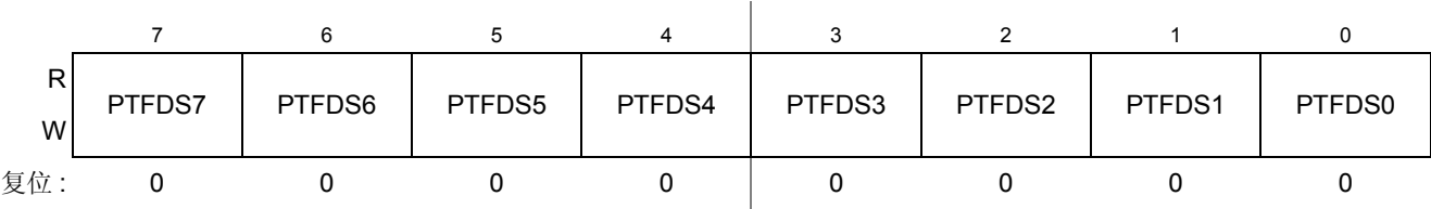
Figure 0-67. F 端口寄存器驱动强度选择 (PTFDS)
