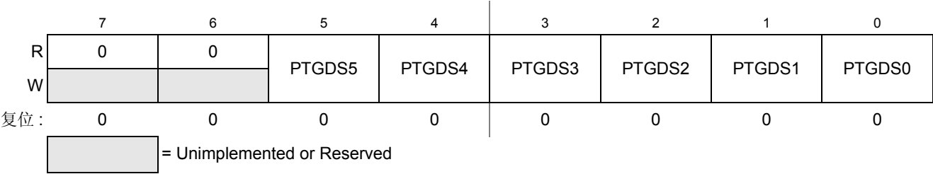
Figure 0-72. G 端口寄存器的驱动强度选择 (PTGDS)
