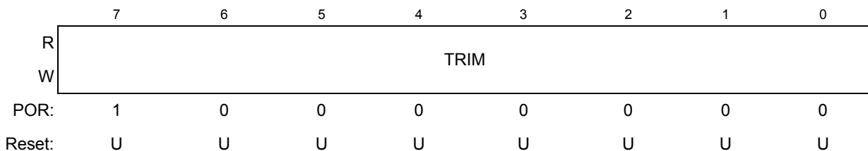
Figure 9-5. MCG 修正寄存器 (MCGTRM)
