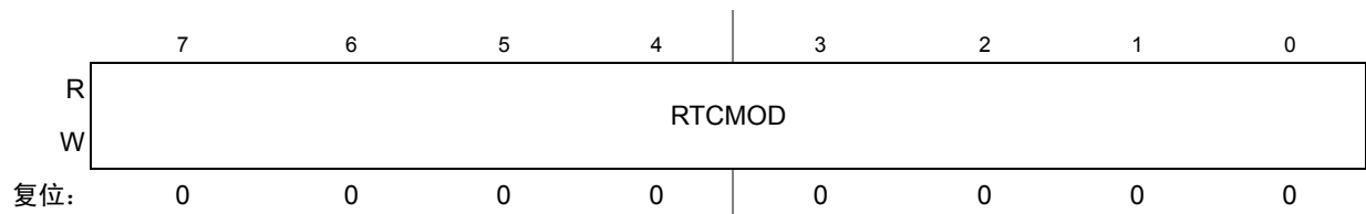
Figure 16-5. RTC 模数寄存器 (RTCMOD)
