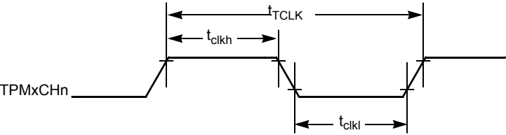
Figure B-5. 定时器外部时钟
