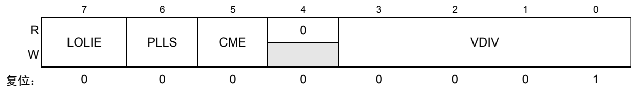
Figure 9-7. MCG PLL 寄存器 (MCGPLL)
