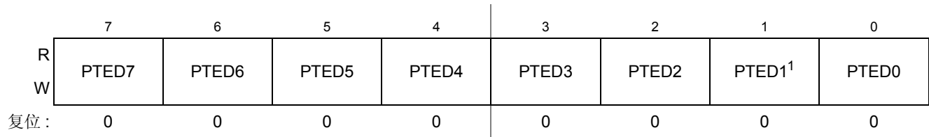
Figure 0-58. E 端口数据寄存器 (PTED)
