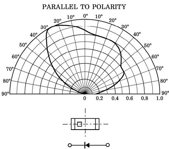
TLSU1002A-2 [RADIATION PATTERN]
