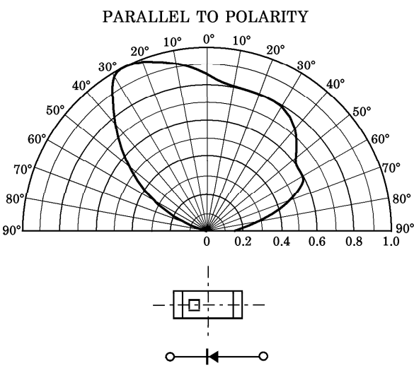
TLGU1002A-2 [RADIATION PATTERN]
