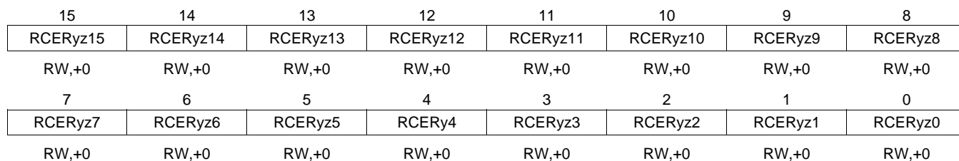
Figure 3-13. Receive Channel Enable Registers Bit Layout for Partitions A to H
