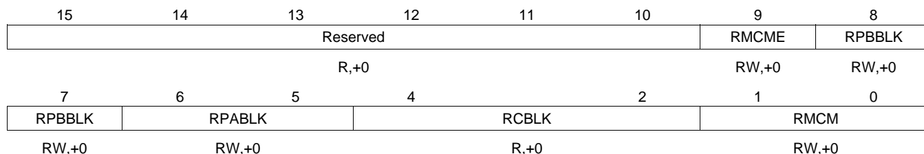
Figure 3-12. Multichannel Control Register 1x (MCR1x)
