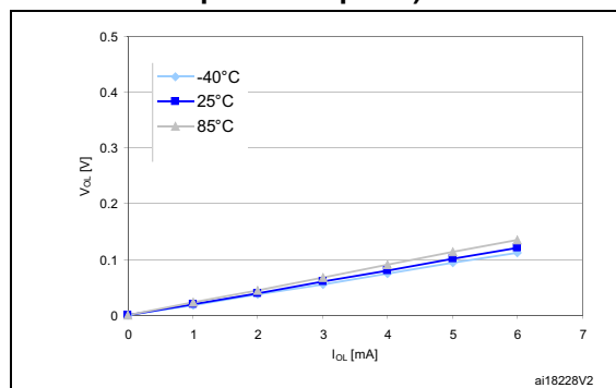
Figure 26. Typical V_{OL} @ V_{DD} = 3.0 \text{ V} (true open drain ports)
