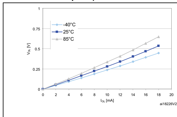
Figure 24. Typical V_{OL} @ V_{DD} = 3.0 \text{ V} (high sink ports)
