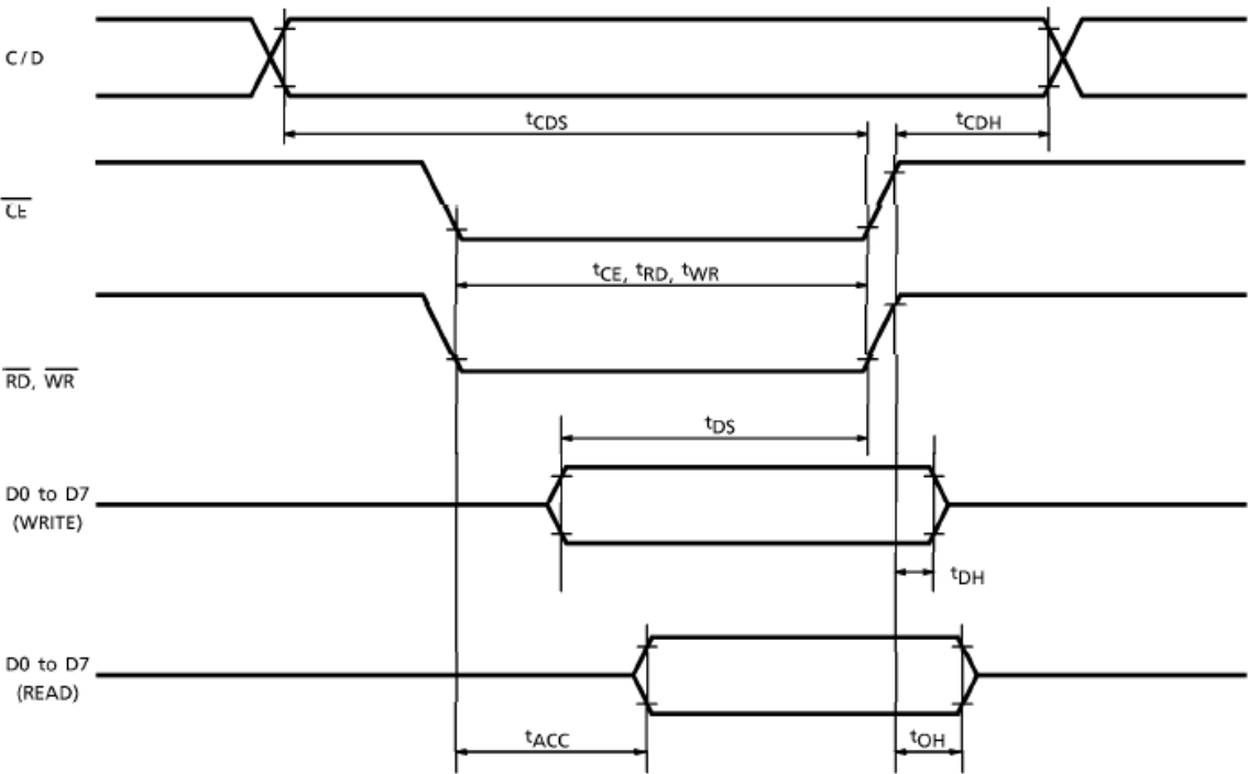
Bus Timing
