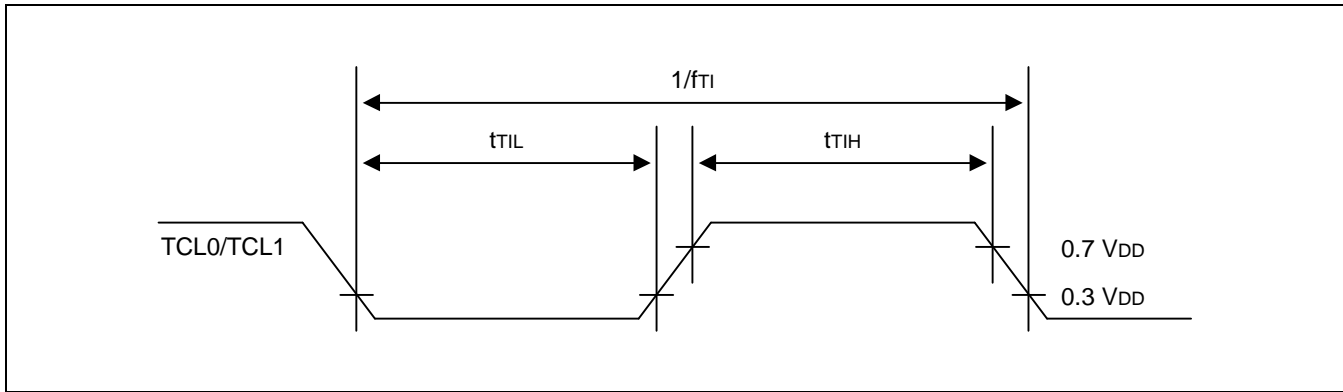
Figure 15-7. TCL0/TCL1 Timing
