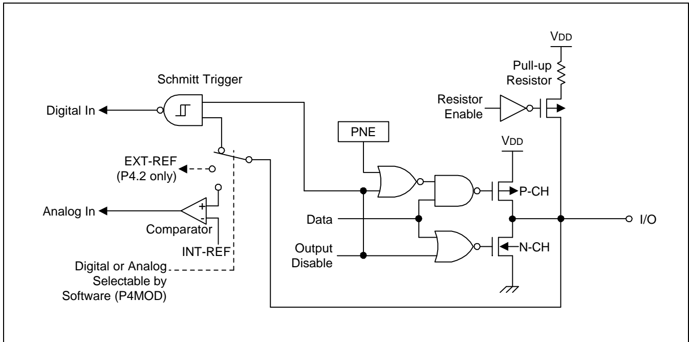
Figure 1-8. Pin Circuit Type F-4
