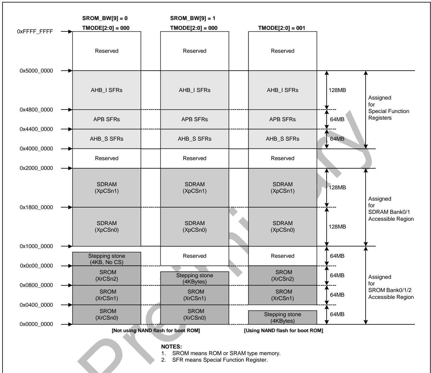
Figure 1-2. Address map
