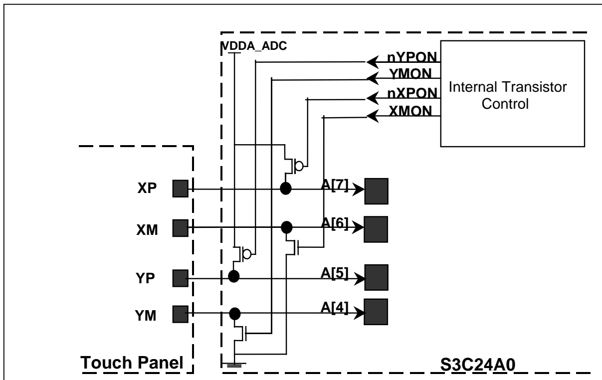
Figure 30-2. Example of ADC and Touch Screen Interface
