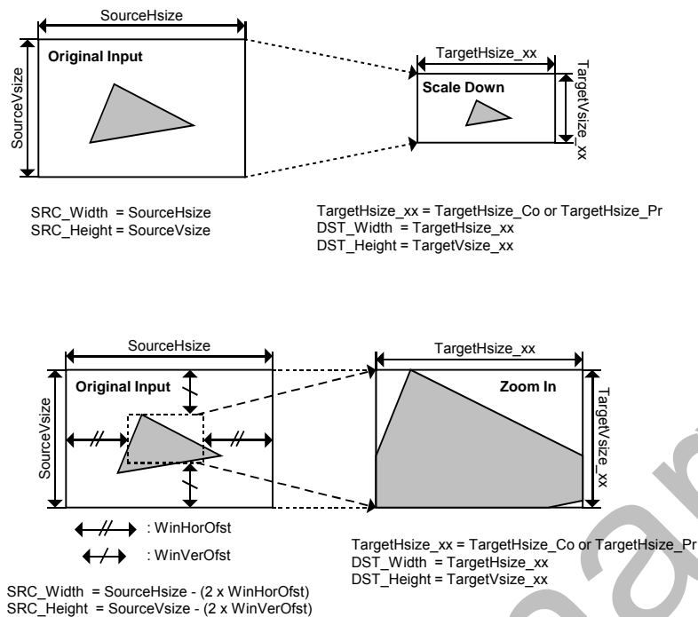
Figure 21-15 Scaling scheme
