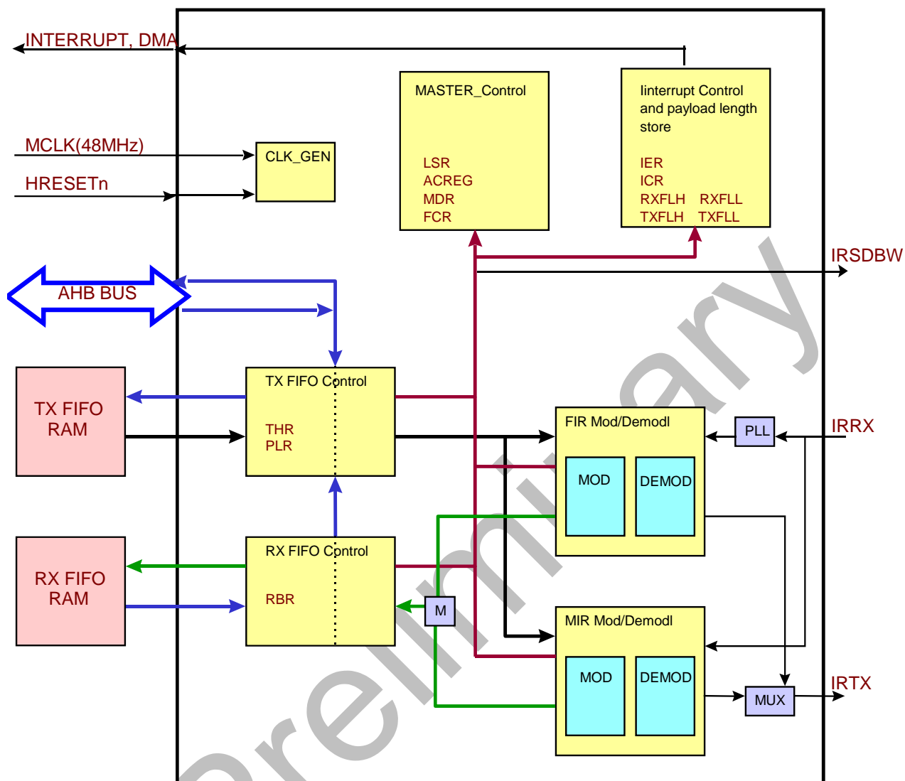
Figure 12-1. Block Diagram
