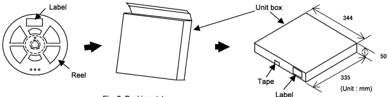
Fig. 6 Packing style
