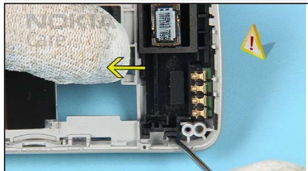
32. Unlock the ANTENNA CELLULAR ASSY.
