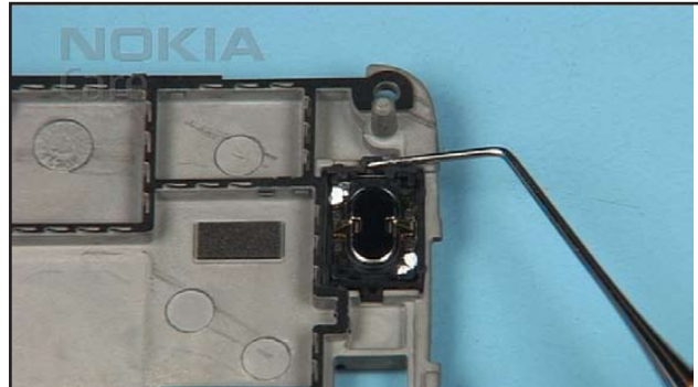
26. Remove the EARPIECE.
