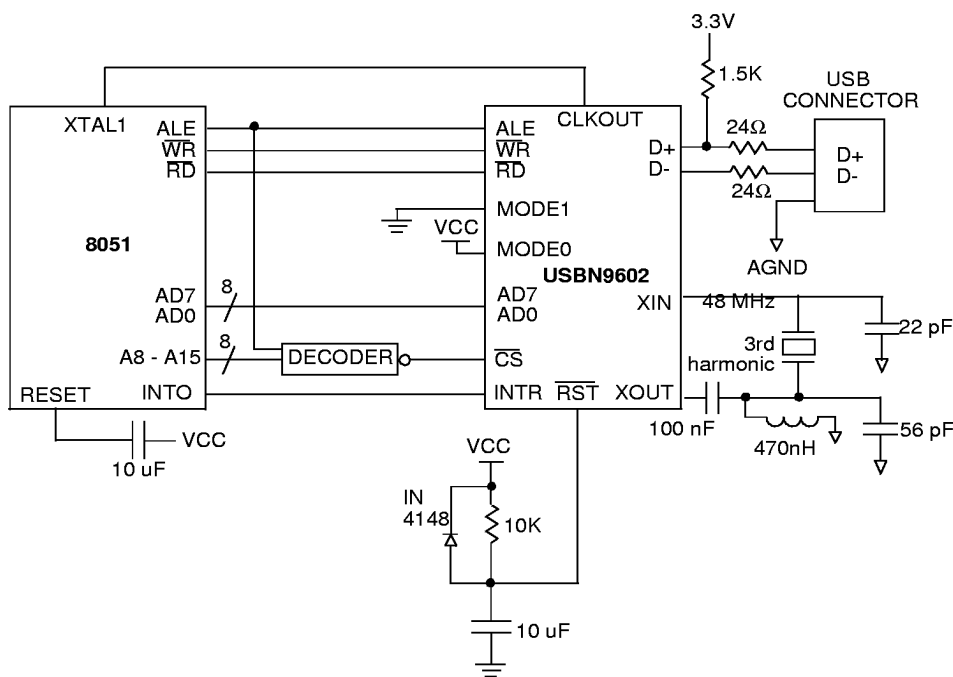
Figure 21. Multiplex Parallel Interface
