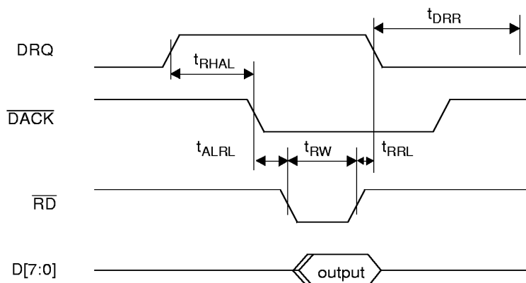
Figure 27. DMA Read to USBN9602
