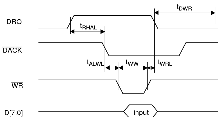
Figure 26. DMA Write to USBN9602
