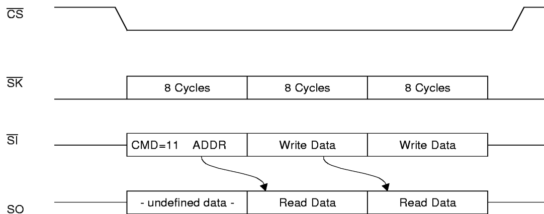
Figure 13. MICROWIRE Interface Burst Write Timing
