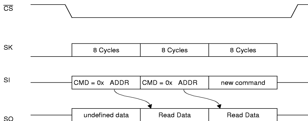
Figure 11. MICROWIRE Interface Basic Read Timing
