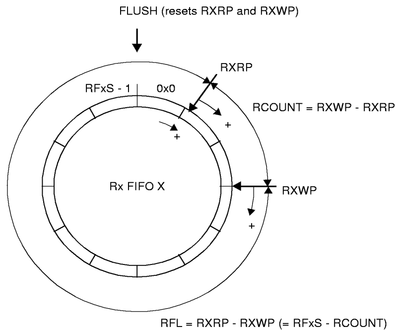
Figure 18. Rx FIFO Operation
