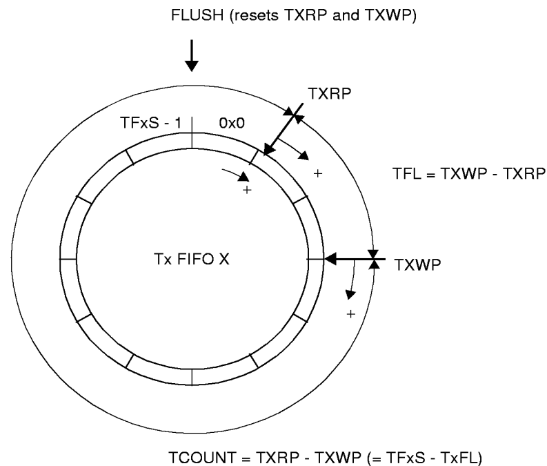
Figure 17. Tx FIFO Operation
