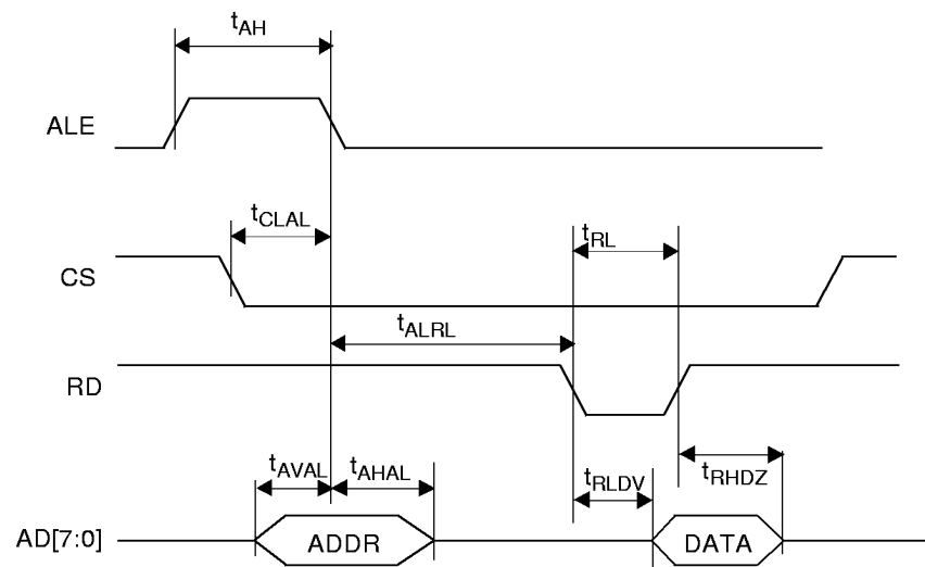
Figure 24. Multiplexed Mode Interface Read Timing
