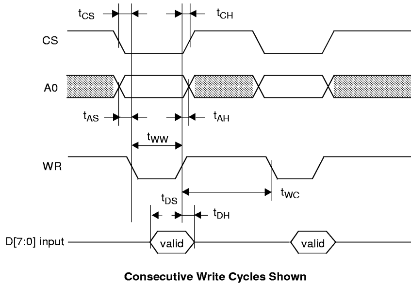
Figure 23. Non-Multiplexed Mode Write Timing
