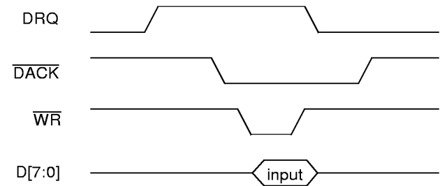
Figure 8. DMA Write to USBN9602
