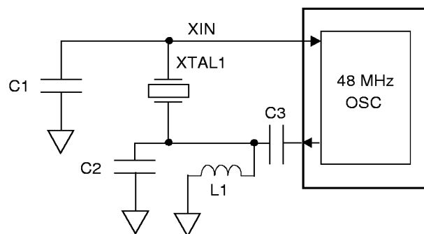
Figure 2. 3rd Harmonic Crystal Oscillator Connections
