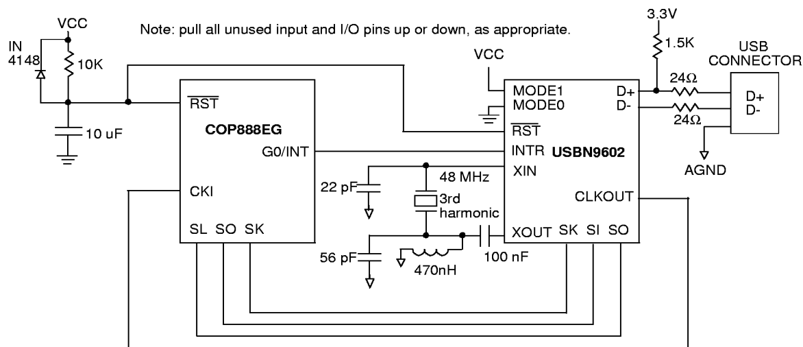
Figure 20. MICROWIRE Serial Interface
