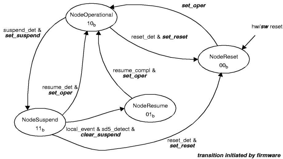
Figure 14. Node Functional State Diagram
