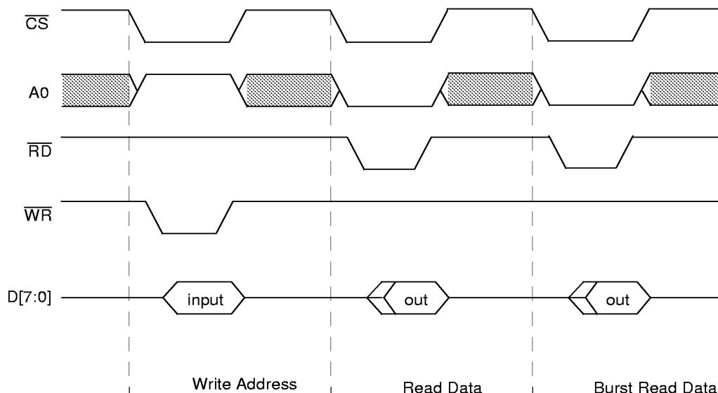
Figure 4. Non-Multiplexed Mode Basic Timing Diagram
