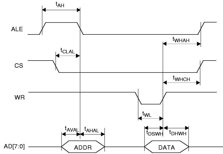
Figure 25. Multiplexed Mode Interface Write Timing
