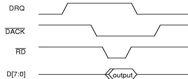
Figure 9. DMA Read from USBN9602
