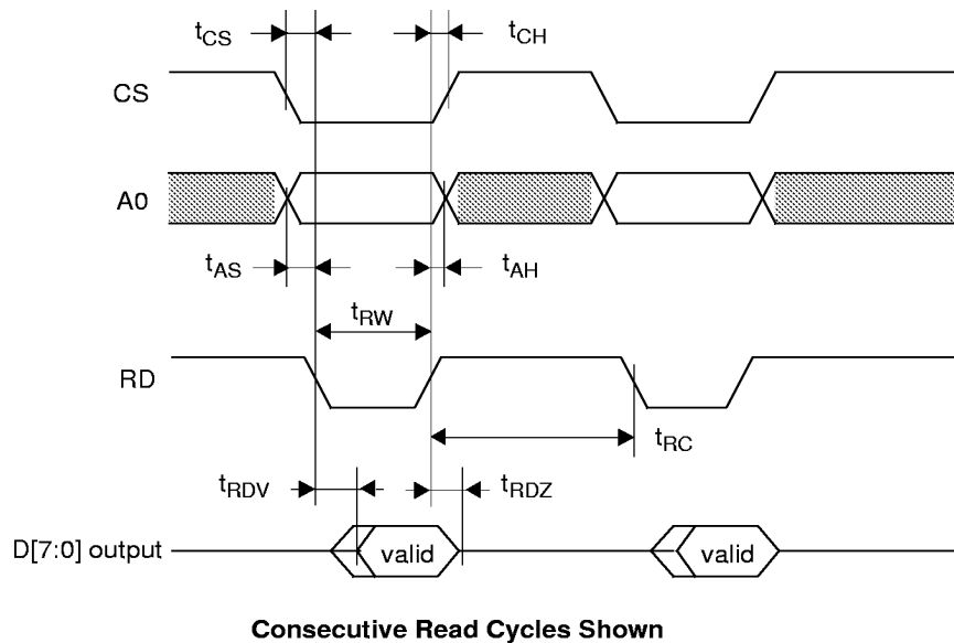
Figure 22. Non-Multiplexed Mode Read Timing
