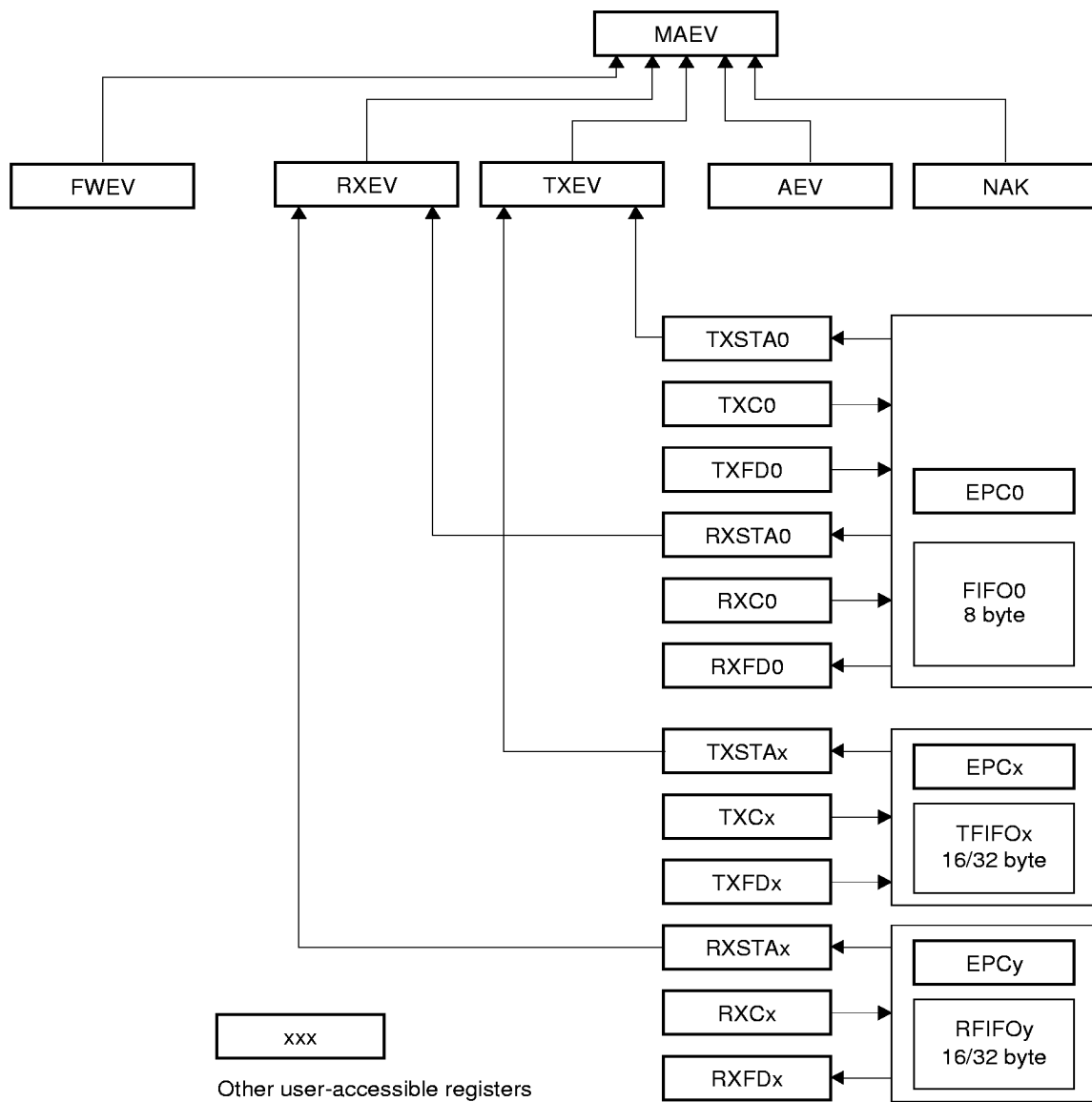
Figure 19. Register Hierarchy
