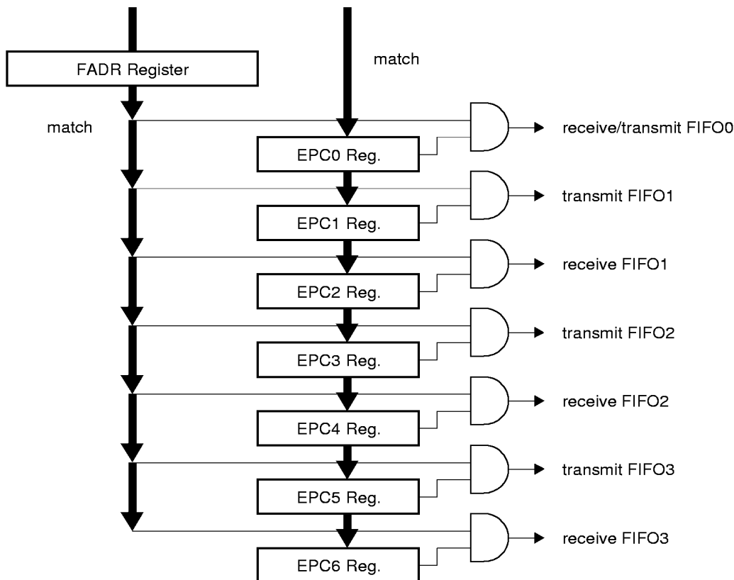
Figure 15. USB Function Address/Endpoint Decoding
