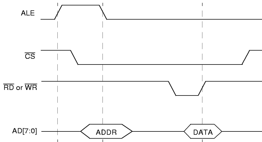
Figure 7. Multiplexed Mode Basic Read/Write Timing
