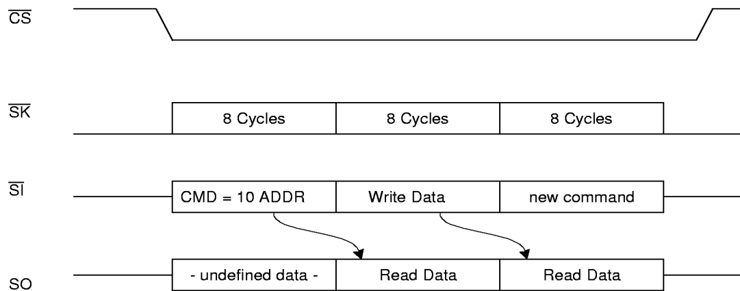
Figure 12. MICROWIRE Interface Standard Write Timing
