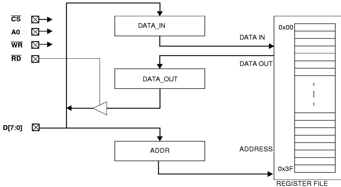
Figure 3. Non-Multiplexed Mode Interface Block Diagram
